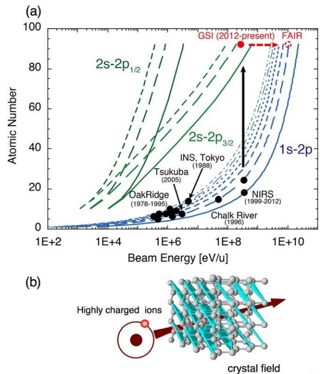
Figure 24. (a) Relationship between beam energy and atomic number required to observe the RCE process. The lines are calculated for the 1s-2p transition in H-like ions, and the 2s-2p_{1/2} and 2s-2p_{3/2} transitions in Li-like ions. (b) Schematic view of highly charged ions passing through a periodic structure of crystals. Reprinted figure with permission from [176], Copyright 2013 by the American Physical Society.
