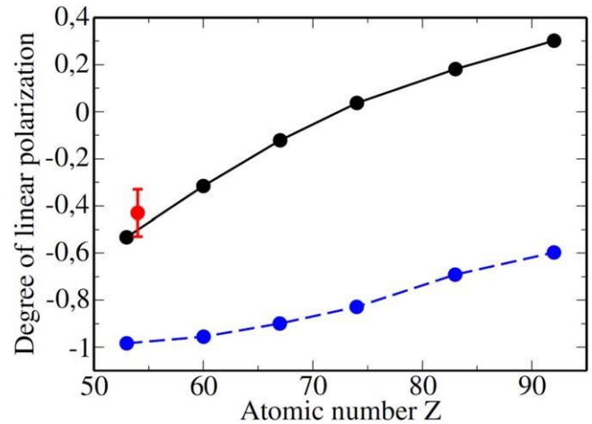
Figure 8. Degree of polarization of the 1s\ 2s^2\ 2p_{1/2}\ J = 1 \rightarrow 1s^2\ 2s^2\ J = 0 emission perpendicular to the incident ion beam.
