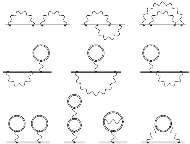
Figure 20. One-electron two-loop Feynman diagrams which contribute to the Lamb shift. The double line represents an electron propagating in the Coulomb field. The wavy line indicates a virtual photon.
