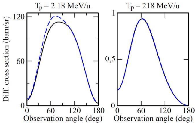
Figure 9. Angle-differential cross sections for the radiative electron capture into the 1s^2 2s^2 ^1S_0 state of (initially) lithium-like uranium ions U^{89+} with projectile energies of 2.18 and 218 MeV/u. Results are presented within the independent particle model (-dashed line) and MCDF approach (solid line). See [69] for further details. Reprinted figure with permission from [69] Copyright 2015 by the American Physical Society.
