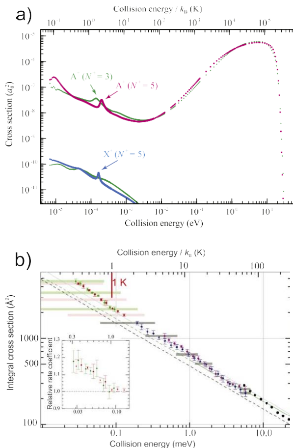
Figure 2. (a) Cross sections of the H^+ + H (green) and D^+ + D (red and blue) radiative association reactions for approach on potentials of the ground ( X^+ ) and first excited ( A^+ ) states (from [13]). (b) Cross section and relative rate coefficient of the H_2^+ + H_2 \rightarrow H_3^+ + H reaction. Black dots [15]; green dashed line [16]; black dashed line (Langevin behavior). Colored dots: merged-beam results from [14].
