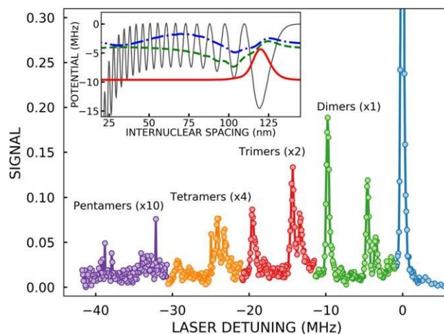
Figure 3. Rydberg excitation spectrum in the vicinity of the 5s38s ^3S_1 strontium Rydberg state. Inset—calculated molecular potential for 5s38s ^3S_1 – 5s^2 ^1S_0 atom pair. Wavefunctions R_C(R) for the v = 0, 1, and 2 molecular vibrational states are included.
