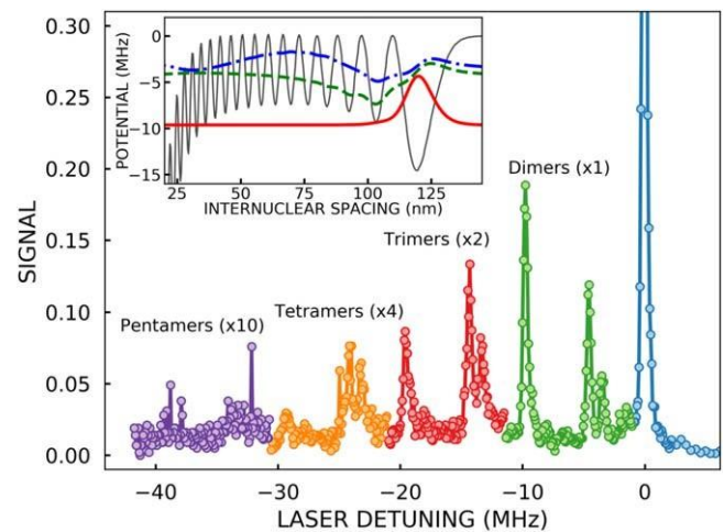
Figure 3. Rydberg excitation spectrum in the vicinity of the 5s38s ^3S_1 strontium Rydberg state. Inset—calculated molecular potential for 5s38s ^3S_1 – 5s^2 ^1S_0 atom pair. Wavefunctions RC(R) for the v = 0, 1, and 2 molecular vibrational states are included.
