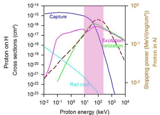
Figure 16. Cross sections of elementary atomic collision processes for the system p \rightarrow \text{H} as a function of the proton energy. The brown line is the stopping power (refer to the right y-axis) for protons in aluminum. The pink area marks the intermediate collision regime.
