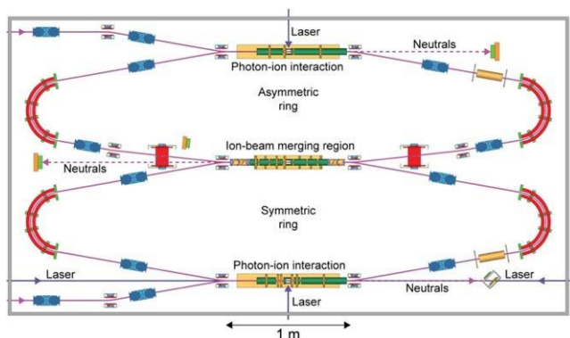
Figure 28. DESIREE [194] at Stockholm University consists of two electrostatic ion-storage rings in a common cryogenic vacuum chamber and with a common straight section where beams of opposite charge polarity can be merged. With the low internal energies that can be attained by waiting for the ions to reach thermal equilibrium and the high degree of control of the inter-particle motion obtained from the merged-beams configuration, unprecedented control of all internal and external degrees of freedom can be obtained.
