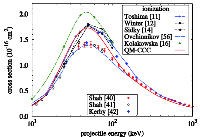
Figure 6. Total ionization cross section for proton-hydrogen collisions as a function of projectile energy. References to indicated previous works are given in [56]. Reproduced with permission from [56]. © IOP Publishing Ltd. All rights reserved.
