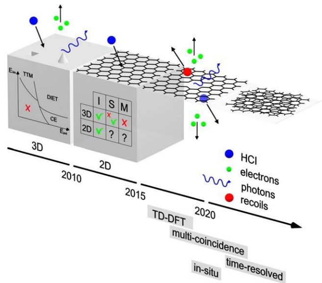
Figure 23. HCI irradiation of surfaces from bulk materials revealed efficient nanostructuring. Possible processes are surface melting (described by TTM), DIET, or Coulomb explosion (CE) depending on the ion's kinetic and potential energies. 3D insulators (I), semi-conductors (S), and metals (M) show different susceptibility to HCI driven modification, whereas further research for 2D materials is needed. In the future, more complex integrated multi-coincidence spectroscopy and in situ microscopy in combination with refined theoretical descriptions will reveal details on the interaction mechanisms.
