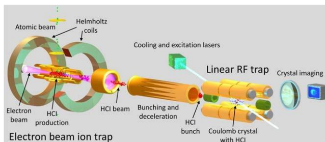
Figure 18. Frequency metrology with HCI: an electron beam ion trap emits HCI that are decelerated, bunched, and injected into a linear radio-frequency trap, where sympathetic cooling with a previously prepared Coulomb crystal of several \text{Be}^+ ions takes place. Then, an ensemble of one single HCI with one single \text{Be}^+ ion is prepared and cooled to its motional ground state. Resonant excitation of forbidden transitions in the HCI, and detection of those excitations by means of quantum-logic spectroscopy follow. In this method, interrogation of the Raman side-band transitions of \text{Be}^+ yields the state of the HCI (Image: MPIK).
