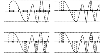
Fig. 1: A^* q_k for the first four iterations.
