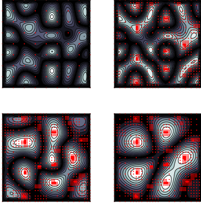
Fig. 2: Evolution of |A^*q_k| and \Omega_k , for (from top left to bottom right) k = 1, 5, 10 and 15 along a run of iterative discretization algorithm. Notice the concentration of grid points near the vertices of the regular pentagon on the circle of radius .5 around the origin (that is, the support of \mu^* ) for late iterations.
