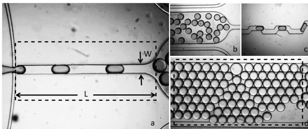
Figure 4. The fabricated flow-focusing assembly, (a) drive channel with width W and length L , (b) droplet generation at 500 \mu\text{L}/\text{h} and 100 \mu\text{L}/\text{h} for drive and dispersed phase, (c) output channel for droplet frequency monitoring, (d) micro-analysis and storage chamber.
