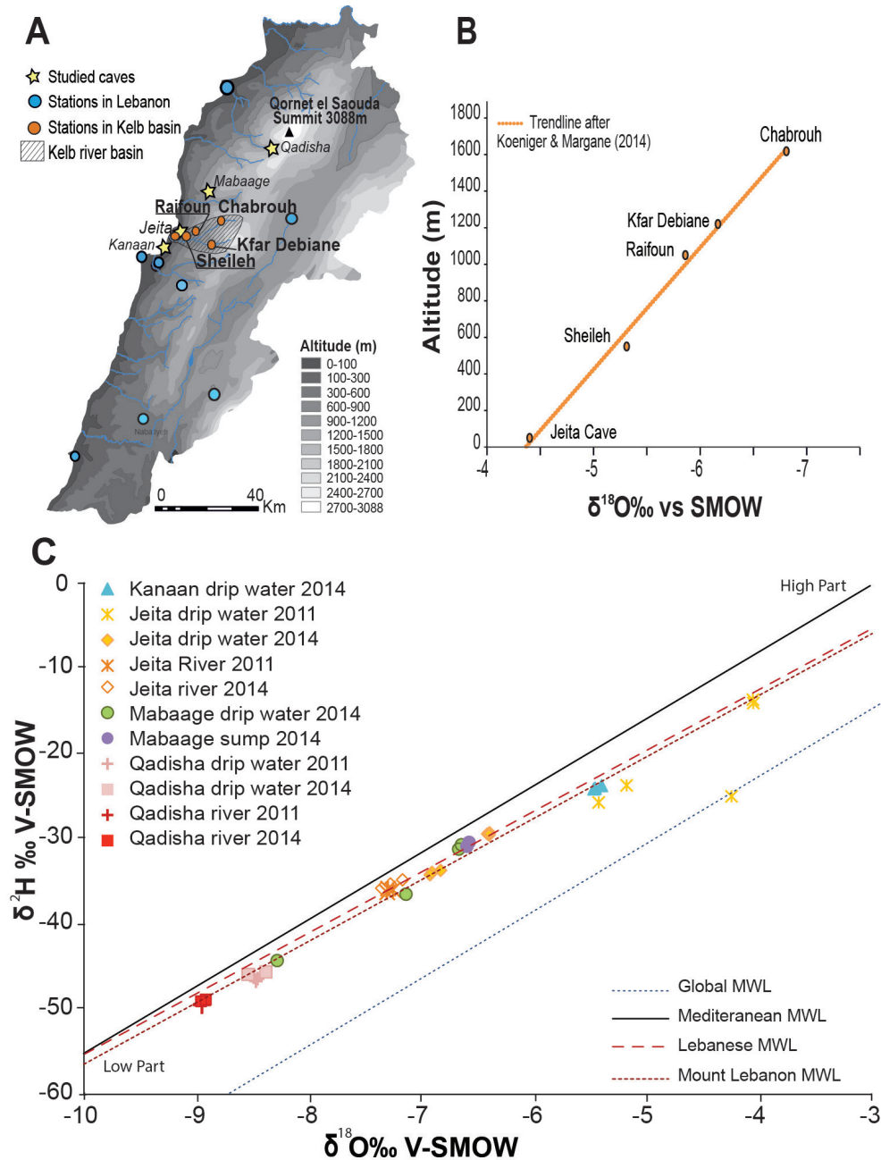
Fig. 4. Summary of major cave drip and stream water \delta^{18}\text{O} and \delta^2\text{H} values plotted on the available meteoric water lines (MWL) with the location of their meteorological stations. A) location of the studied caves (yellow stars) and the meteorological stations (blue circles) in Saad et al. 2005 and Saad & Kazpard, 2007 and (orange circles) in Koeniger & Margane, 2014; B) the altitudinal trendline used in this study and derived from the Local MWL of 222 the Kelb basin (Koeniger & Margane, 2014); C) \delta^{18}\text{O} and \delta^2\text{H} values of 47 dripwater and stream samples plotted on the available MWLs.
