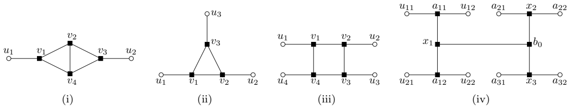
Figure 3: Configurations needed for proving Theorem 1.4. Black square vertices are distinct vertices whose full neighborhood is part of the configuration. White circle vertices are (not necessarily distinct) vertices that might have other neighbors outside the configuration.
