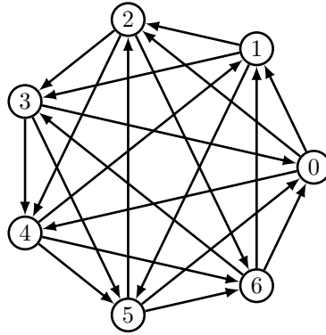
Figure 1: The Paley tournament \overrightarrow{\text{Pal}}_7 on seven vertices.
