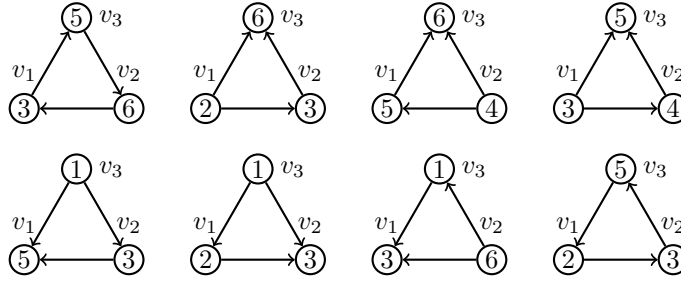
Figure 5: The 8 orientations of the inner cycle induced by \{v_1, v_2, v_3\} .
