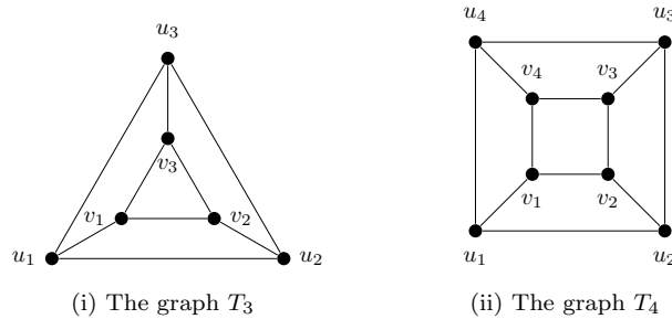
Figure 4: Two cubic graphs mentioned in the proof of Theorem 1.4.
