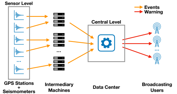
Figure 2: High-level architecture and data workflow for the Earthquake Early Warning System.
