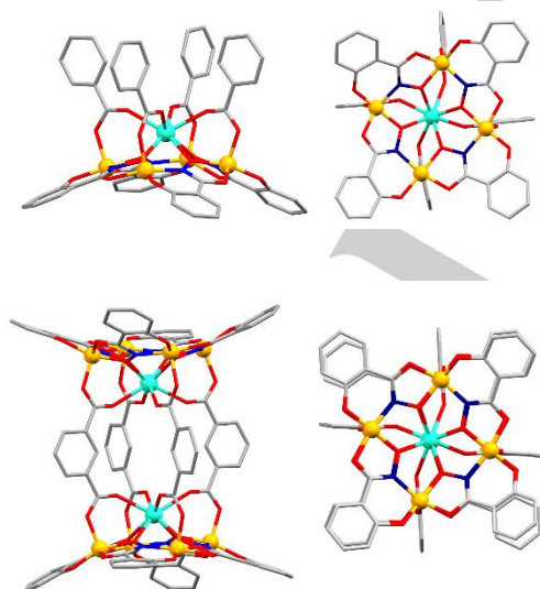
Figure 2. Structures of \text{DyGa}_4 MC (top) and [\text{DyGa}_4]_2 dimeric complexes (bottom) obtained from X-ray diffraction on single crystals: (left) side-view and
