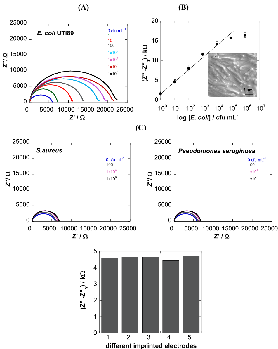
Fig. 3. (A) Nyquist plots of E. coli imprinted electrodes upon exposure to E. coli UTI89, (B) Calibration curve: inset: SEM image of the interface after rebinding; (C) Nyquist plots of E. coli imprinted electrodes upon exposure to S. aureus and Pseudomonas aeruginosa (D) Reproducibility of the sensor fabrication tested upon the incubation with 100 \text{ cfu mL}^{-1} E. coli UTI89.
