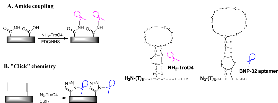
Figure 5: Presentation of the construction of an immunosensor: (A) Amide coupling for the generation of a sensor specific for cTnI proteins (MW=24 kDa); (B) Use of “click chemistry” for the integration of a BNP-32 aptamer for the sensing of BNP-32 peptide (MW=3.4 kDa).
