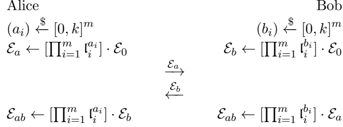
Figure 11: The Commutative Supersingular Diffie–Hellman key exchange
