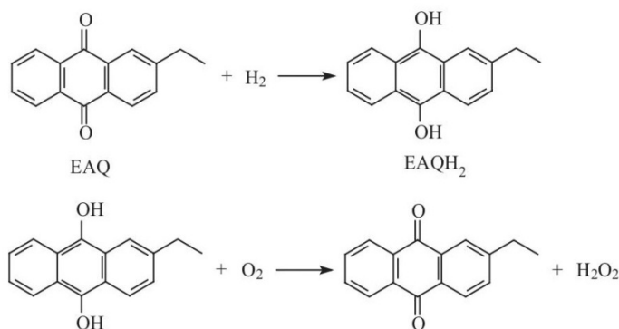
Fig. 11. Two-stages of hydrogen peroxide synthesis [8]
