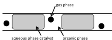
Fig. 10. Flow pattern of GLL in channel [6].
