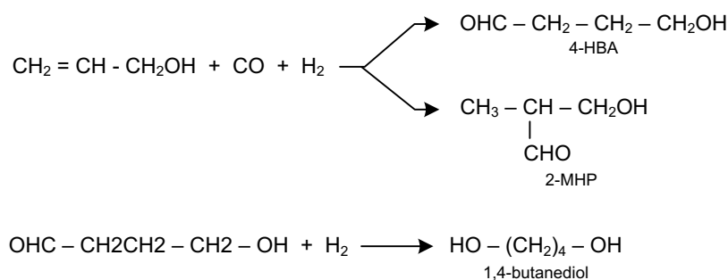
Fig. 7. Hydroformylation scheme of allyl alcohol [24]
