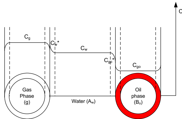
Fig. 2. Schematic diagram of the mass transfer of component C from the gas bubble via the continuous water phase to an oil droplet and possible concentration profiles (Model 1)
