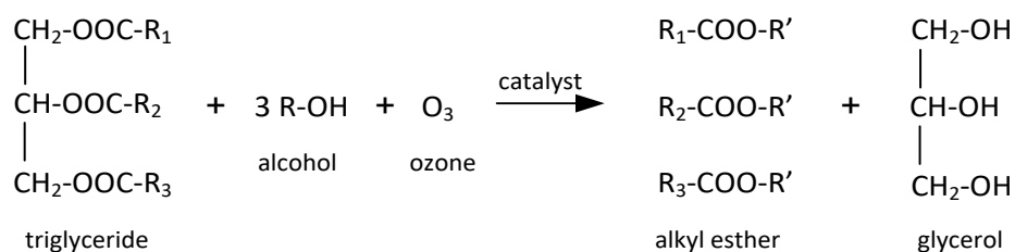
Fig. 6. Ozonolysis scheme for biodiesel production.
