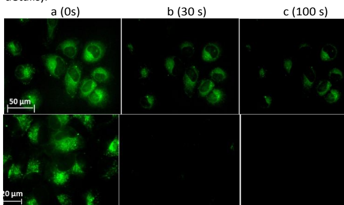
Fig 4 Photobleaching experiments (epifluorescence microscopy) performed on HeLa cells incubated during 1h 30 min with a 95 \mu\text{M} solution of compound 6e (top) or with 50 nM LysoTracker Green DND-26 (bottom) after exposure to the continuous excitation light at 414 nm, band pass 46 nm filter during different times: (a) 0 s, (b) 30 s, (c) 100 s. 63 \times objective.
