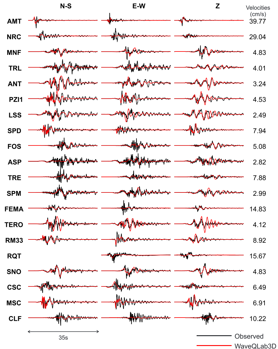
Figure 10. Comparison between observed (black) and synthetic (red) velocity waveforms for the best-fitting model of Figure 4 calculated by WaveQLab3D in frequency range 0.05–5.0 Hz. Note that there is no additional alignment time shift of the individual waveforms.
