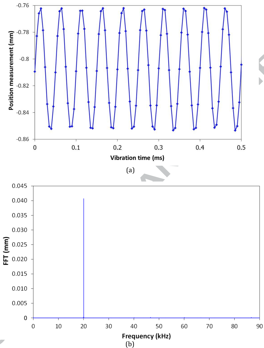
Figure 12: (a) Representative example of the measured sonotrode displacement using a laser sensor at position 1 (as shown in Figure 11) with a nominal amplitude of 45.4 \mu\text{m} . (b) Corresponding Fast Fourier Transformation (FFT).
