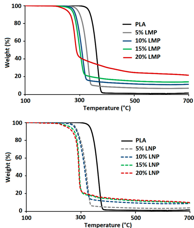
Figure 9. Effect of lignin size and content of PLA thermal stability during TGA under nitrogen.
