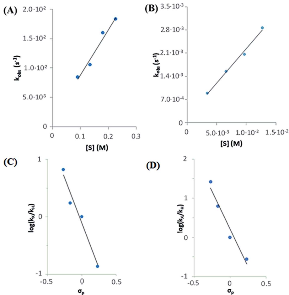
Fig. 9 Top: rate dependence on substrate concentration of reactions of (A) 1^{(\text{IV})}=\text{NTs} (left) with \text{MeO}^{\text{PhSMe}} substrate (denoted as [S] ) and (B) 2^{(\text{IV})}=\text{NTs} with \text{MeO}^{\text{PhSMe}} substrate (right) at 293 K. Bottom: Hammett plot representing \log(k_x/k_H) against Hammett parameter ( \sigma_p ) for the reactions of (C) 1^{(\text{IV})}=\text{NTs} (left) and (D) 2^{(\text{IV})}=\text{NTs} (right) with p -X-thioanisoles in acetonitrile at 293 K. k_x values correspond to the second order rate constants obtained by measuring k_{\text{obs}} values at different p -X-thioanisole concentrations.
