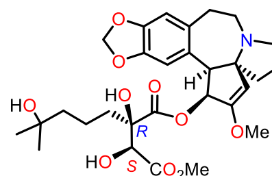
57 Cephalozimine E (0.0001%)*
