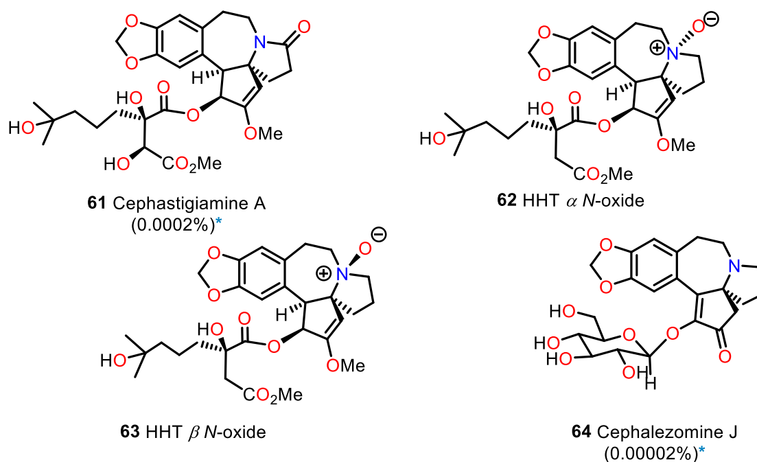
Figure 11. Oxygenated Cephalotaxus esters and Cephalezomine J
