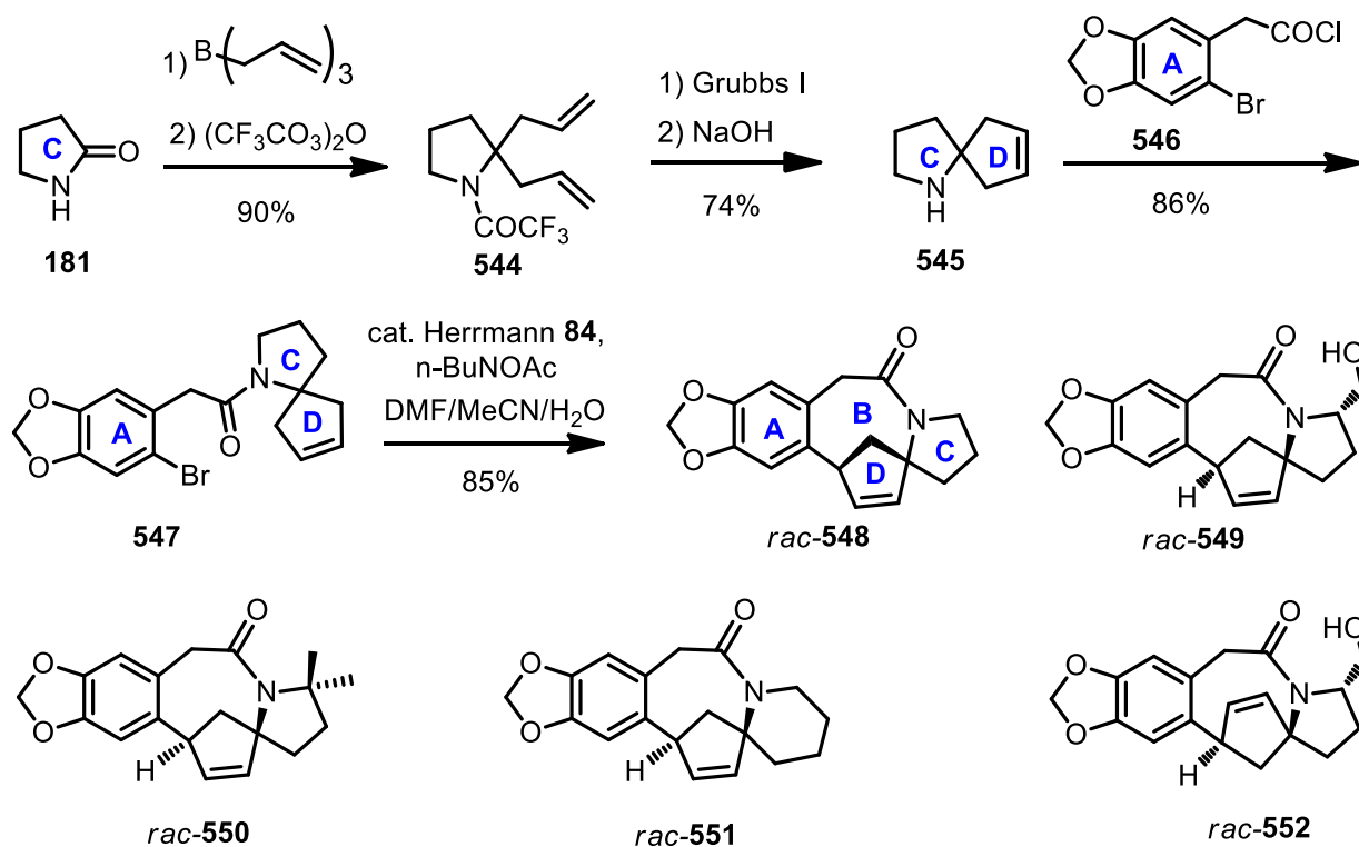
20 Scheme 59 CET's analog synthesized by Bubnov (2005-2010)
