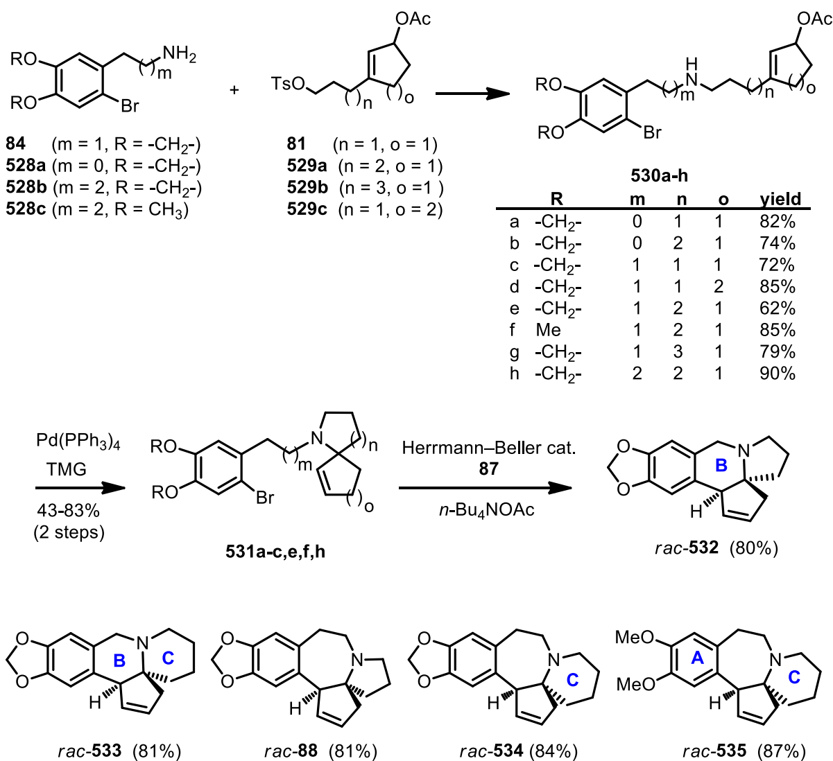
Scheme 57 Synthesis of CET analogs by Tietze (2000)
