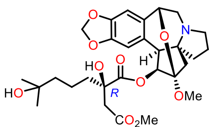
53 Cephalozimine A (0.0001%)*
