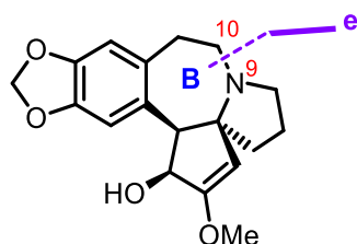
Figure 17. N9–C10 bond disconnection e for construction of CET (1) B ring
