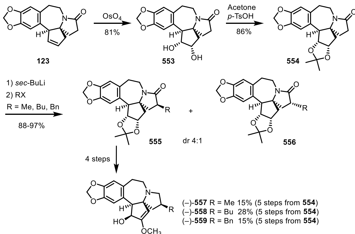
10 Scheme 60 Synthesis of CET alkylated analogs by Royer (2004)
