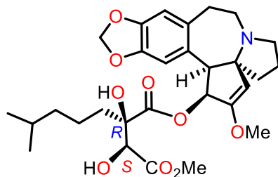
58 Cephalozimine F (0.002%)*
