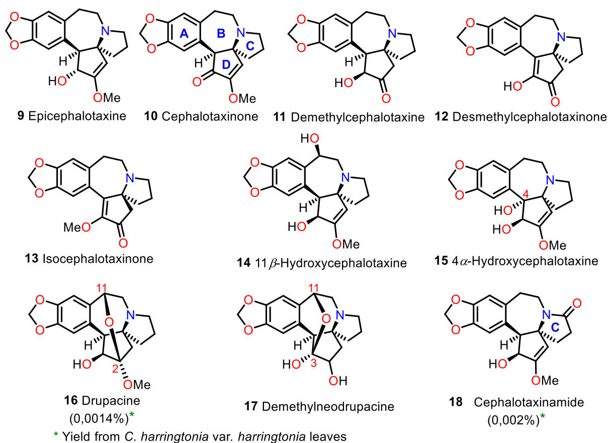
Figure 4. Oxydized cephalotaxines
