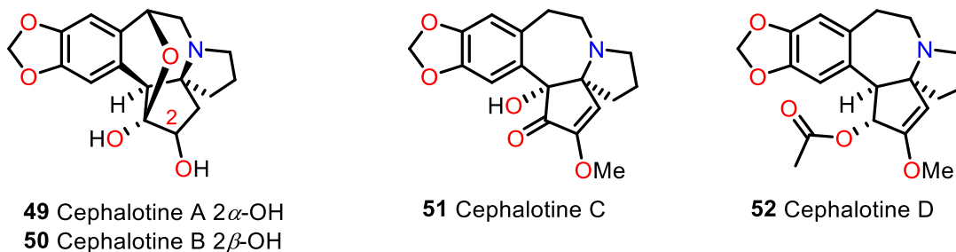
Figure 9 Cephalotines A-D
