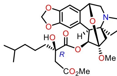
54 Cephalozimine B (0.00005%)*
