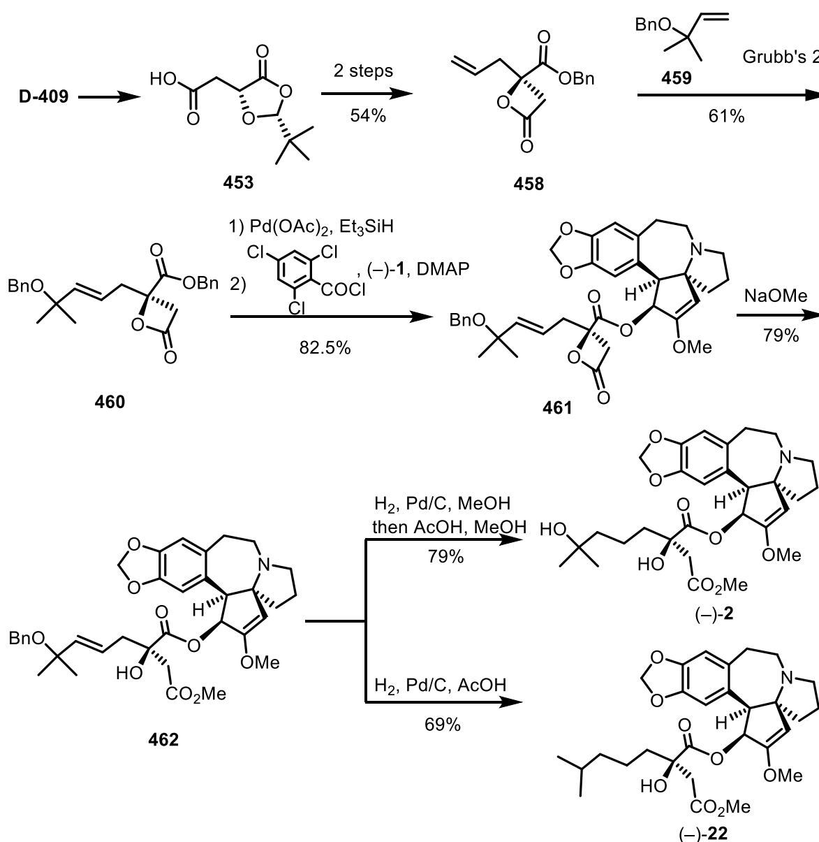
Scheme 49 Synthesis of HHT (-)-(2) and homodeoxyHT (-)-(22) by Djaballah and Gin (2008)
