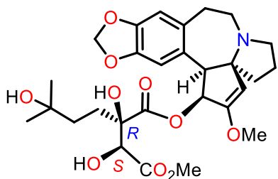
55 Cephalozimine C (0.002%)*
