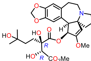
56 Cephalozimine D (0.0003%)*
