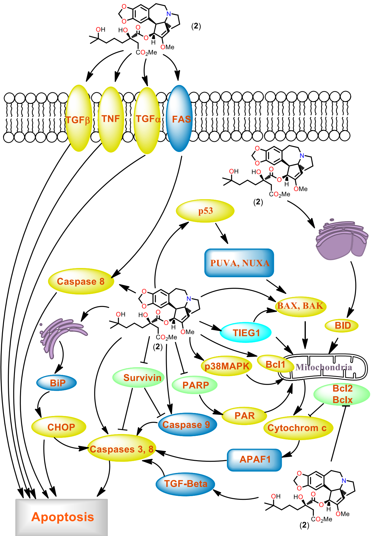
Figure 26: Main pathways involved in apoptosis mechanism induced by HHT (2). Yellow: apoptosis factor; Blue: apoptosis intermediary; Turquoise: Dual role as intermediary and factor; Green: Apoptosis inhibitor
