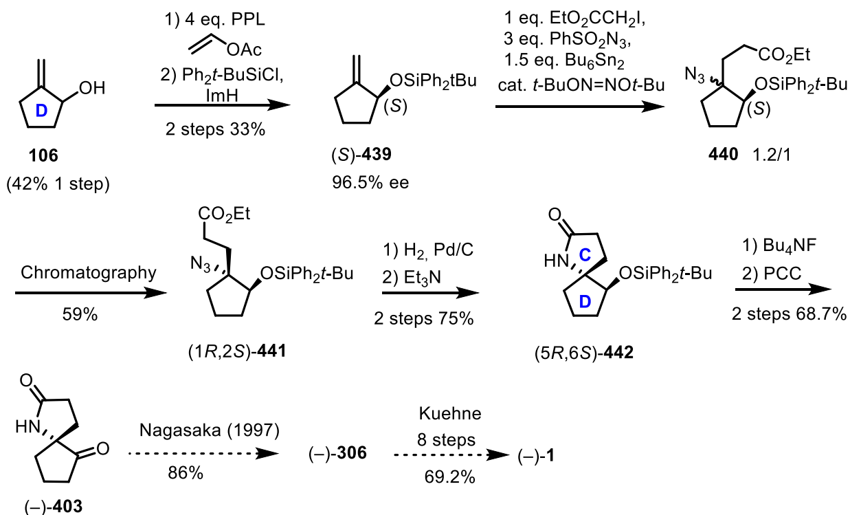
5 Scheme 43. Formal asymmetric synthesis of CET (-)- 1 via Nagasaka's intermediate by Renaud (2012)
