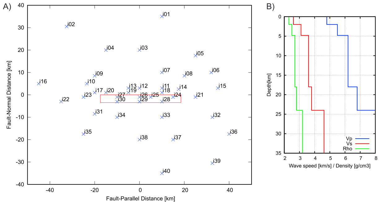
Figure 2. (a) Geometry of fault (red box) and station locations (crosses) of the source inversion validation (SIV) test Inv1. The right-lateral strike-slip fault dips at 80^\circ and reaches the surface. (b) Parameters of the 1-D elastic layered medium that is considered in calculation of the Green's functions.
