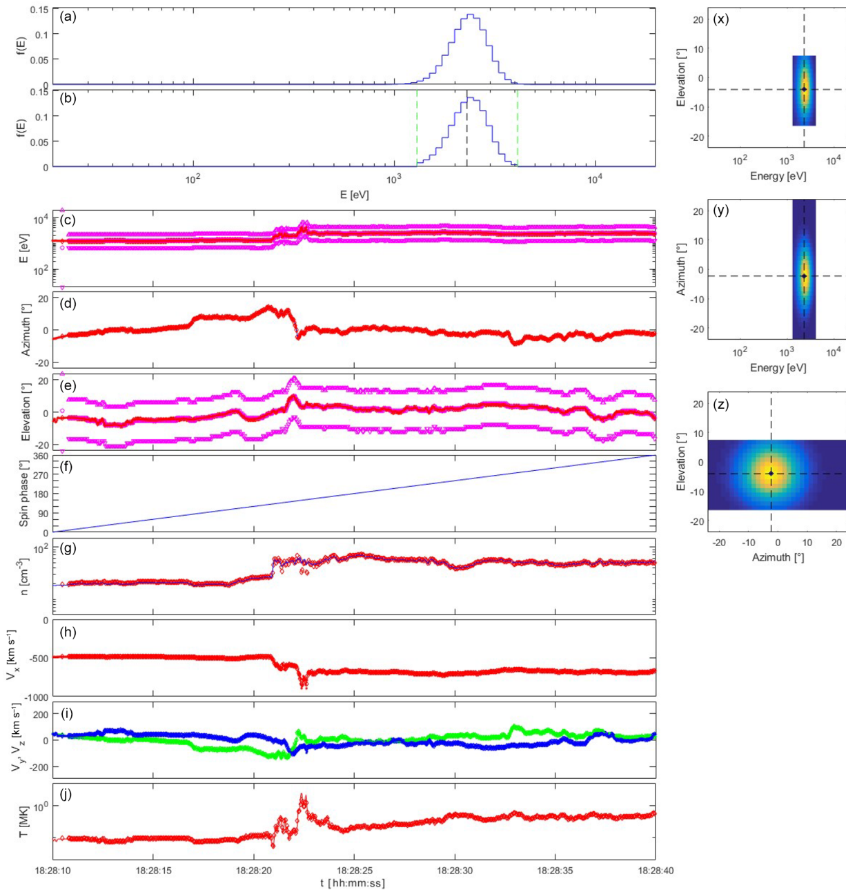
Figure 8. Plasma spectrometer measurements for a solar wind simulation based on Spekt-R/BMSW observations of a strong shock on 22 June 2015, using internal energy and elevation beam tracking. The plot layout is the same as that of Fig. 7.
