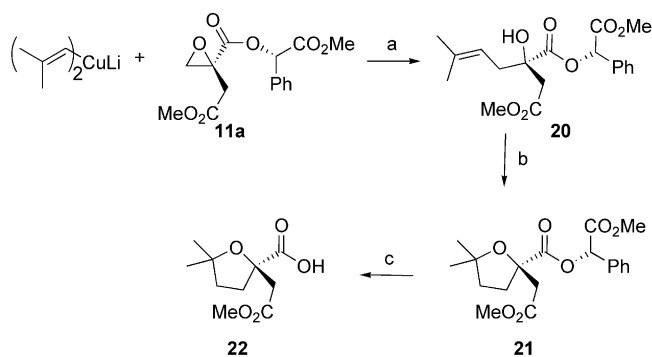
Scheme 4. Synthesis of anhydroharringtonine monoacid side-chain from epoxide 11a . Reagents and conditions: (a) Et 2 O, -78 to -60 °C, 2 h (55%); (b) Hg(OAc) 2 , NaBH 4 , THF/H 2 O, 0 °C to room temperature, 2.5 h (76%); (c) H 2 , Pd/C, AcOEt, room temperature, 5 h (90%).
