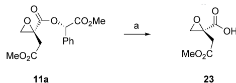
Scheme 5. Hydrogenolysis of epoxide 11a . Reagents and conditions: (a) H 2 , Pd(OH) 2 , THF, room temperature, 2 h (70%).
