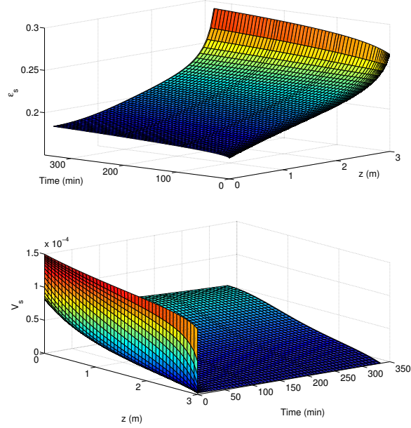
Figure 5. First 3D simulation of solid phase volume fraction \epsilon_s and solid particles velocity V_s .
