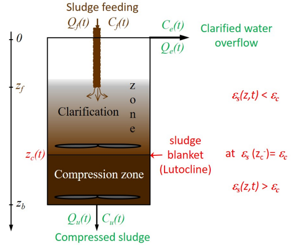
Figure 1. One-dimensional schematic view of a Settling Tank.
