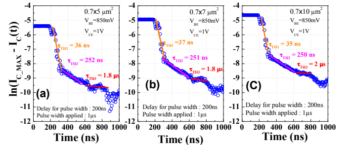
Figure 12: Extraction of thermal time constant, \tau_{TH} , from pulse measurements for the geometries with W_{E0}=0.7\mu\text{m} and L_{E0} (a) 5, (b) 7 and (c) 10 \mu\text{m} .
