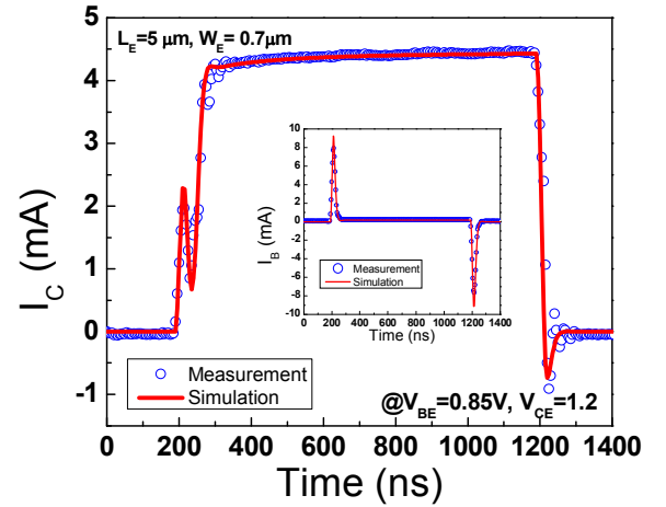
Figure 11: Comparison between measurements (symbols) and simulation (solid lines) of the collector current evolution as a function of the time for V_{BE}=0.85\text{V} and V_{CE}=1.2\text{V} .
