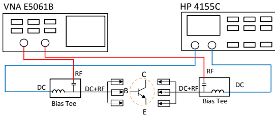
Figure 1: Low-frequency S-parameters measurement setup
