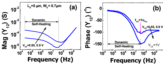
Figure 2: Magnitude and Phase of the parameter Y_{12} depicting distinct regions of self-heating.
