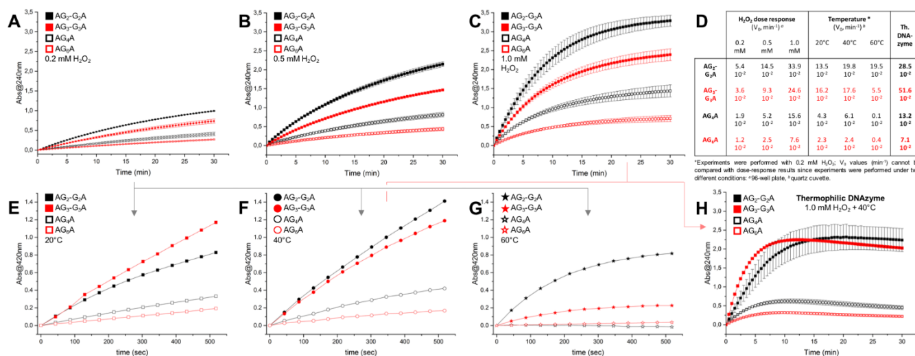
Fig. 5. DNAzyme results of experiments performed with 1 \mu M G4 (the modified AG 2 -G 2 A and AG 3 -G 3 A and their unmodified counterparts AG 4 A and AG 6 A), 1 \mu M hemin, 2 mM ABTS and increasing amounts of stoichiometric oxidant H 2 O 2 (from 0.2 to 1.0 mM, A-C) at 20°C, or with 0.2 mM H 2 O 2 with increasing temperature (from 20 to 60°C, E-G). Optimized thermophilic DNAzyme was designed with 1 \mu M G4, 1 \mu M hemin, 2 mM ABTS, 1.0 mM H 2 O 2 at 40°C (H). All experiments are performed in either 96-well plates (A-C, H) or quartz cuvettes (E-G). See Supporting Information for details. Initial velocity V 0 values (min -1 ) are summarized in table D.
