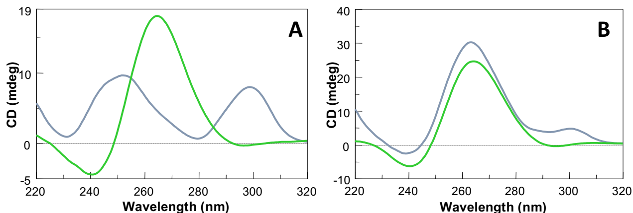
Fig. 4. CD profiles of A ) AG 4 A (green) and AG 2 -G 2 A (blue); and B ) AG 6 A (green) and AG 3 -G 3 A (blue) (70 \mu M, 40 mM K + , 20°C).
