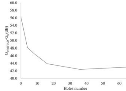
Figure 19. Receptance (dB) decrease between damped and undamped laminates.
