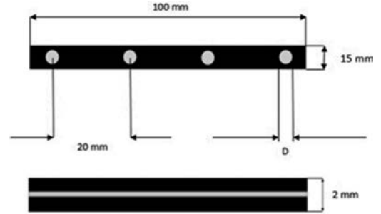
Figure 5. Dimensions of bending test samples.
