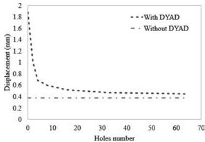
Figure 15. Holes influence on displacement.
