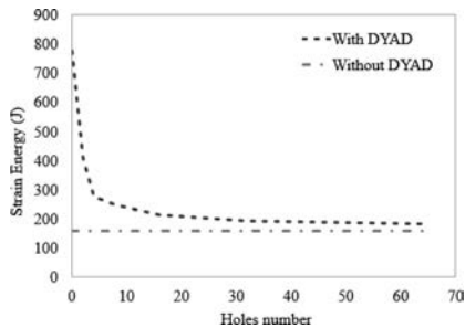
Figure 16. Holes influence on strain energy.
