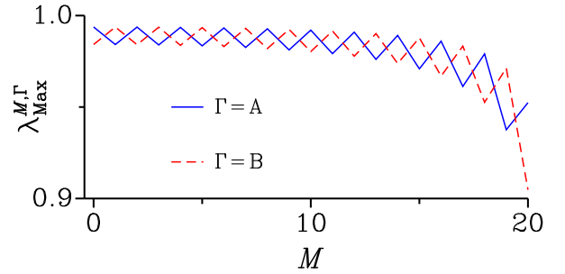
Figure 1. The largest eigenvalue \lambda_{\text{Max}}^{M,\Gamma} of the direction cosine \Phi_{Zx} as a function of M for J_{\text{Max}} = 20 . A solid (dashed) line corresponds to the C_2 symmetry species A ( B ).
