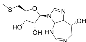
5'-Methylthioformycin
