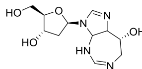
2'-deoxycoformycin
