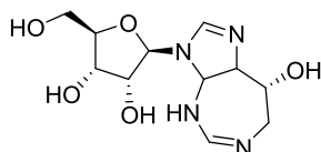
Coformycin
