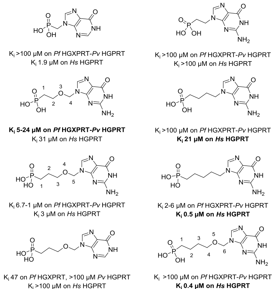
Figure 18: Studies of the impact of the chain length of ANPs on their inhibitory activities against
