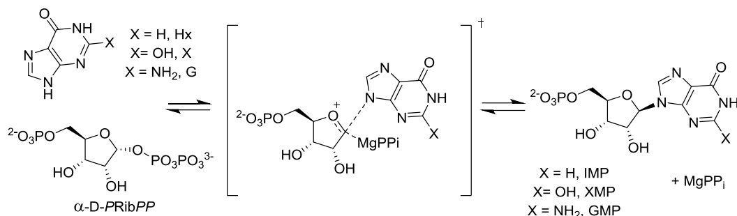
Figure 6: Mechanism and transition state of the 6-oxopurinephosphoribosyltransferase catalyzed reaction
