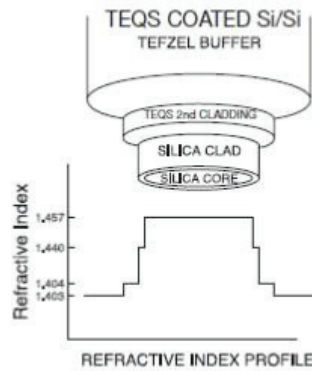
FIGURE 4. (a) Step refractive indexes of a TEQS TM coated multimode fiber. (b) Spheroid tip of 200 \mu\text{m} TEQS TM coated multimode fiber
