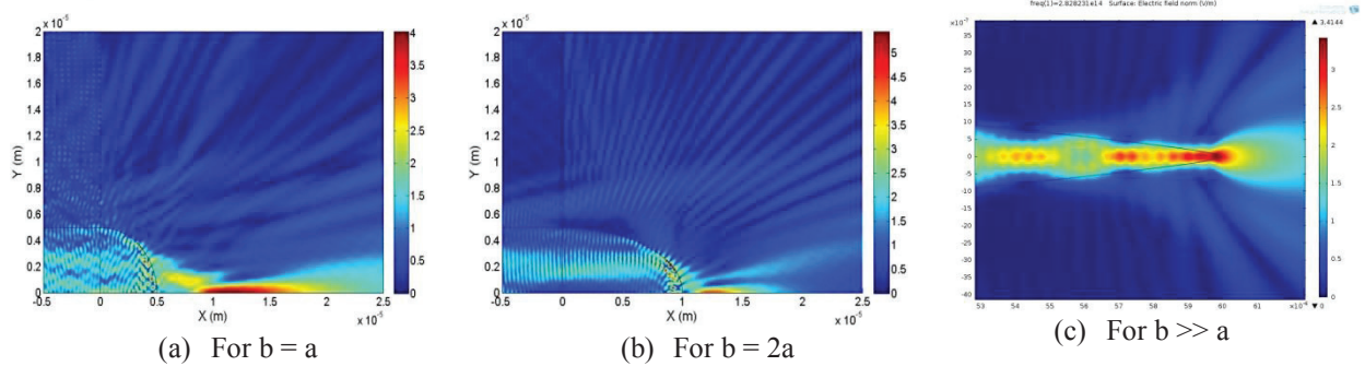
FIGURE 3. PJs generated by 10 \mu\text{m} plane waveguide for the case of tip shape to be (a) circular with axis ratio b=a , (b) elliptical with axis ration b=2a and (c) pointed with axis ratio b \gg a
