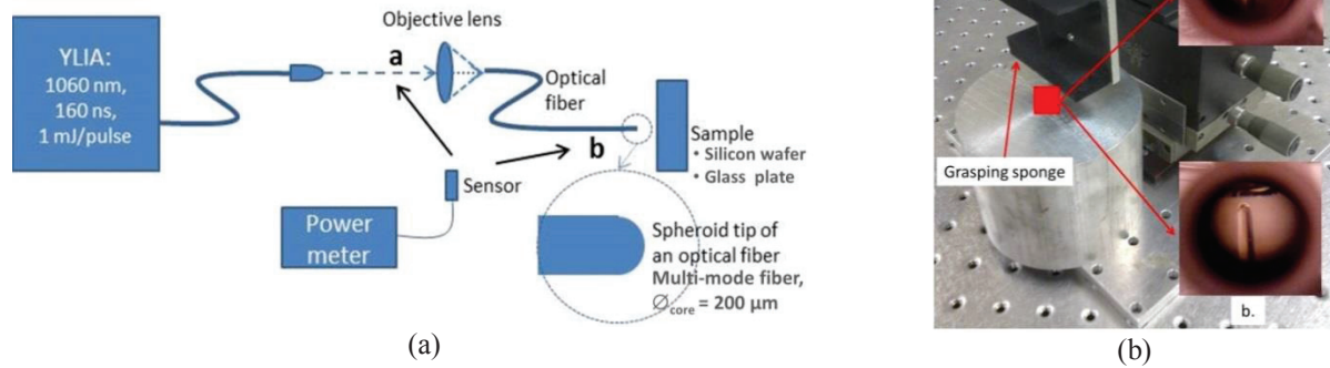
FIGURE 5. (a) Experiment scheme for PJ etching using spheroid tip fiber optics; the sensor at position (a) and (b) is for the laser beam and PJ measurement, respectively. (b) A three-axis micro stage is used to give a space between
