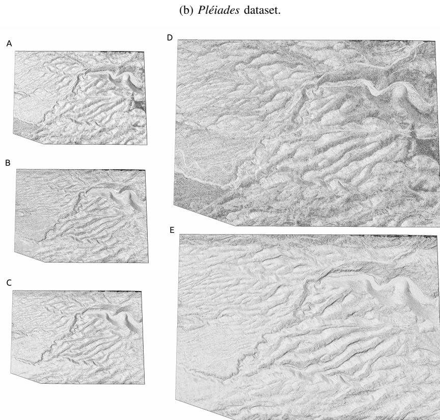
Figure 8: Grayshaded representation of surfaces reconstructed with different methods and at different resolutions. A. CORR_{Z_2} , B. 1Pix_{Z_2} , C. 12Pix_{Z_2} , D. CORR_{Z_1} , E. 12Pix_{Z_1} .
