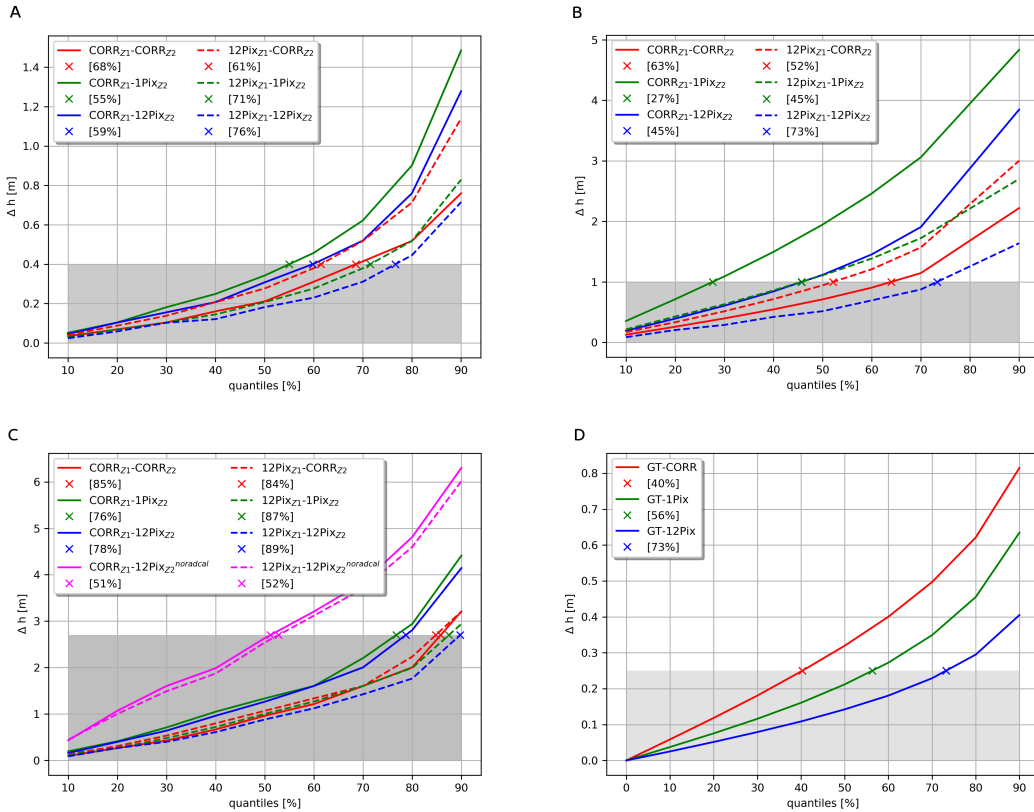
Figure 4: Sample quantiles calculated on: A. Vahingen, B. Pleiades, C. Spot-7, D. Chang'E 3 datasets. The gray zone indicates |\Delta h| values that are \leq GSD (of the lower resolution images). The \times markers correspond to sample quantiles for respective GSD values, i.e., they signal the percent of all \Delta h for which \langle 0 \geq |\Delta h| \leq GSD \rangle .
