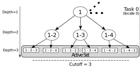
Figure 2: Initial search that generates the active set A for jobs = 4 and cutoff = 3 . The figure depicts the branch that has the element 1 of the permutation as the root and generated 6 valid and feasible incomplete solutions at depth cutoff = 3 .
