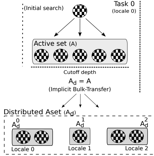
Figure 3: Task 0 is responsible for distributing the active set across several locales. The distributed active set A_d consists of several sets A_d^i, i \in \{0, \dots, L - 1\} , where L is the number of locales on which the application is going to run.
