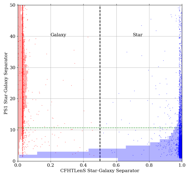
Figure 6. PS1 SGS is plotted against the CFHTLenS star galaxy separator, CLASS_STAR . When the CLASS_STAR is larger than 0.5, it is considered as a star; otherwise, a galaxy. The green dotted line indicates the PS1 SGS limit. The semi-transparent histograms are the respective number counts as functions of PS1 SGS, the full range of the x-axis corresponds to a number count of 2,500.
