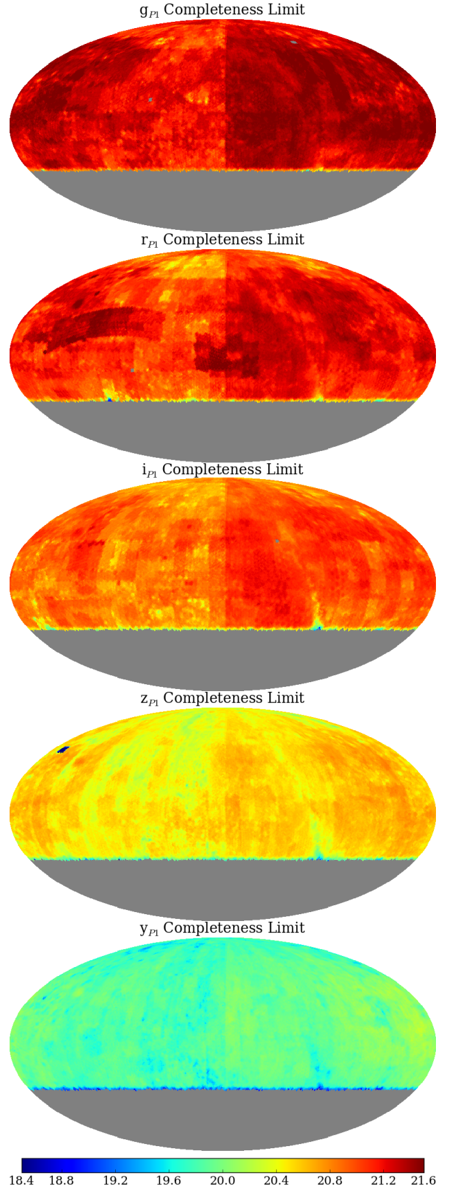
Figure 5. Completeness map in g_{P1} , r_{P1} , i_{P1} , z_{P1} and y_{P1} filters respectively, all magnitudes are with the same colour scale.
