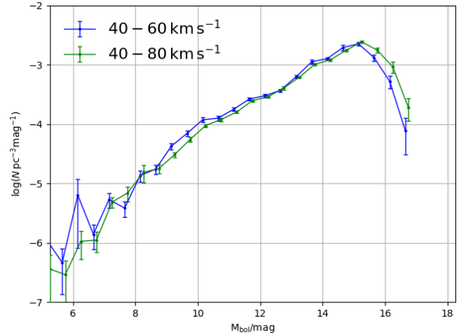
Figure 10. WDLF of the low velocity samples in the solar neighbourhood. The 40–80 \text{km s}^{-1} line is shifted by 0.1 mag for easier visual comparison. The two samples agree well with each other.
