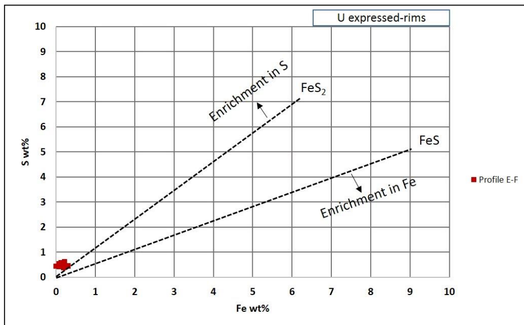
Figure 12. EPMA S and Fe concentration measurements of profile E-F performed on a telohuminitic particle (ulminite). Both S and Fe are always below 1 wt %, with a slight enrichment in S. Reference lines refer to the stoichiometry of FeS 2 (pyrite) and FeS (i.e., mackinawite).
