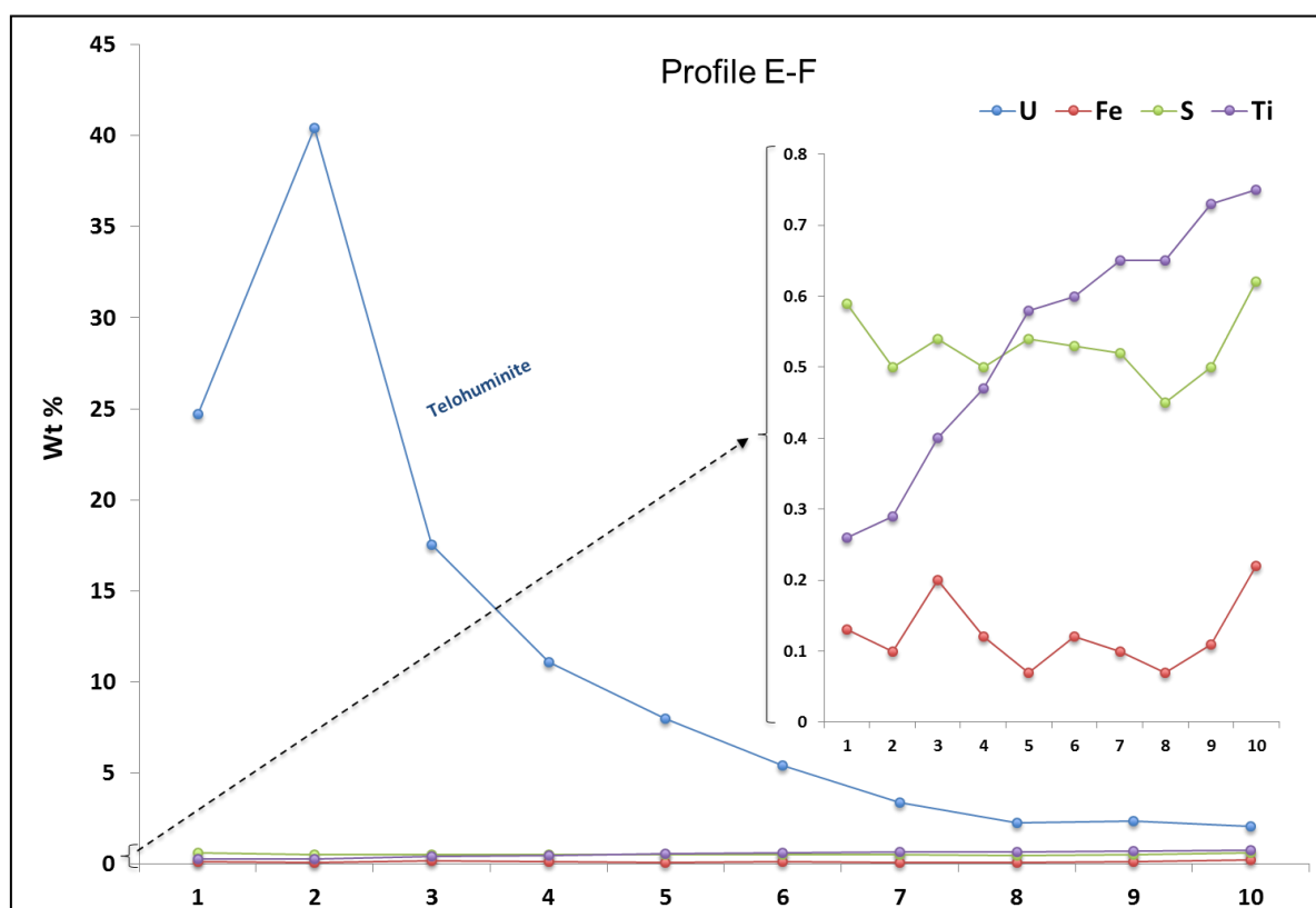
Figure 11. Profile E-F was performed on a telohuminite particle with uranium expressed as \text{UO}_2 at the rims. U concentration starts at 25 wt % at the rim. As shown in Figure 10F, the first point was measured on a part of the particle where \text{UO}_2 is not expressed as uraninite. The next spot was measured on a part where U is expressed as uraninite, hence the concentration is raised to 41 wt %. Afterwards the U concentrations decrease proportionally as a function of increasing distance from the particle rim. The Fe and S concentrations are at 0.1 and 0.5 wt %, respectively (with a detection limit of 0.1 wt %), as shown in the upscaled part of the graph. Titanium concentration increases from the rim towards the interior of the particle, from 0.26 to 0.75 wt %.
