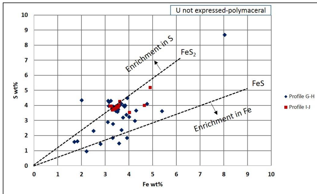
Figure 7. S-Fe binary plot, illustrating profiles G-H and I-J presented in Figure 5. Reference lines refer to the stoichiometry of \text{FeS}_2 (pyrite) and \text{FeS} (i.e., mackinawite).
