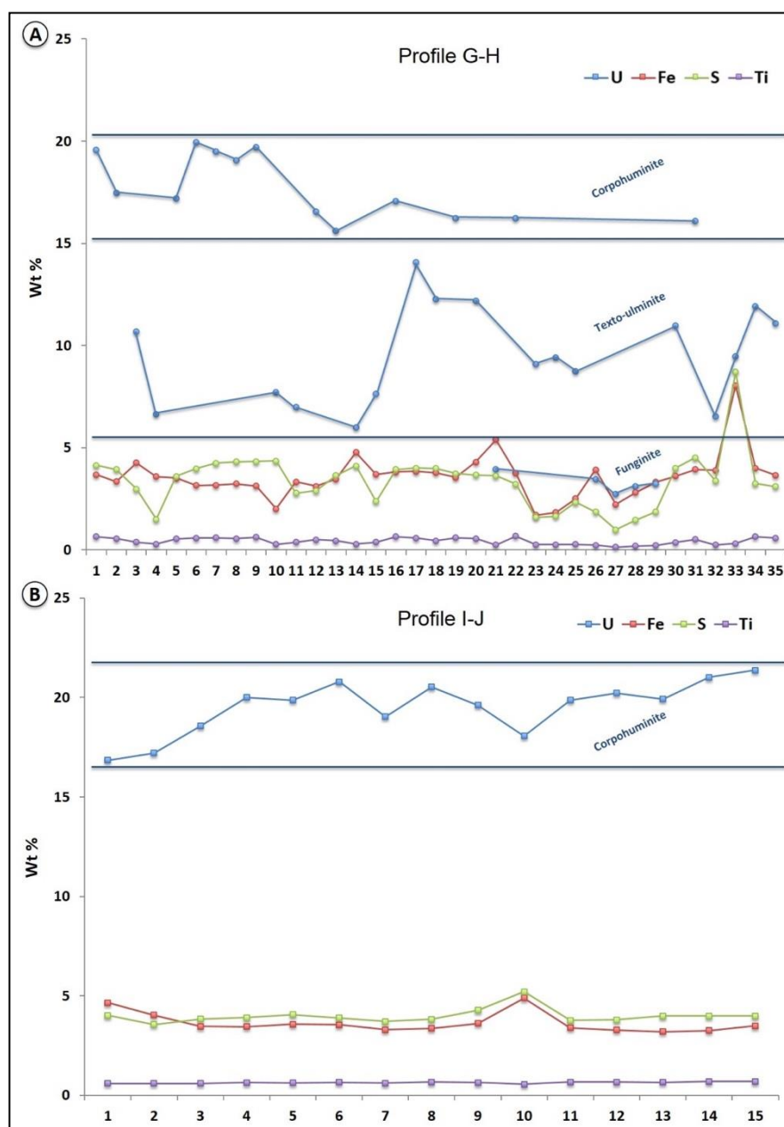
Figure 6. The profiles G-H and I-J presented in Figure 5. Profile G-H (A) indicates that the composition of uranium in corpohuminite is more than double that of the texto-ulminite background, reaching 19 wt %. Sulfur and iron concentrations are not perfectly correlated and several datapoints show antagonistic behavior. Profile I-J (B) was performed on a single corpohuminite particle and shows that uranium concentration is between 16 and 22 wt %. Sulfur and iron are sub-constant and correlated, which could be related to pyrite nanocrystal inclusions. Titanium is sub-constant and around 1 wt % for both profiles.
