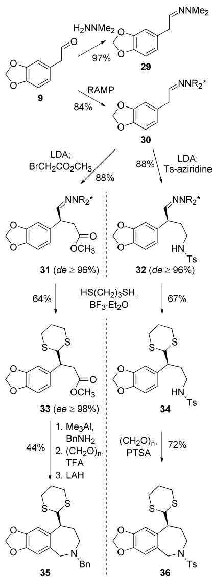
SCHEME 4. Investigations on Route b or Retrosynthesis I
