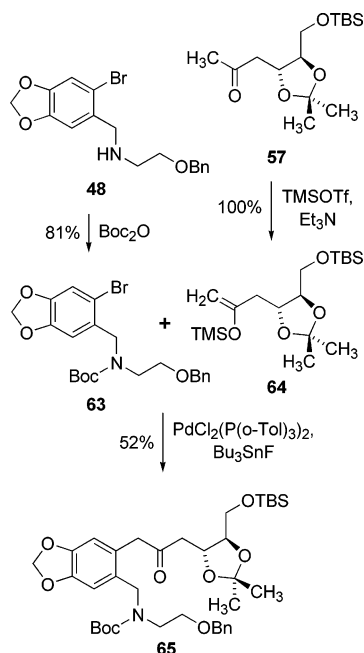
SCHEME 13. Intermolecular Coupling of 63 and 64 According to Kuwajima and Urabe
