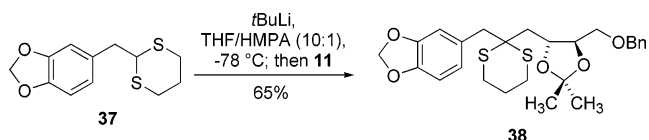
SCHEME 5. Dithiane 37 Was Used To Optimize the Reaction Conditions for Coupling with 11
