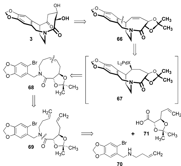
SCHEME 14. Retrosynthesis IV with a RCM and an Intramolecular Heck Reaction as Key Steps
