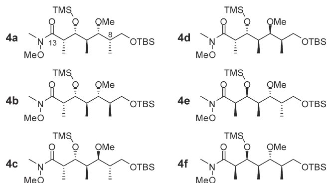
FIGURE 3. Structure of the six diastereomers 4a–f .
