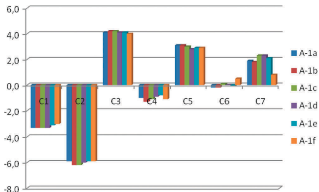
FIGURE 4. Δδ 13 C (ppm) between A and 1a–f for carbons 1 to 7.
