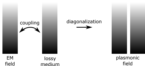
FIG. 1. Spectral structure of the plasmon-polariton model before and after diagonalization. The two continuous spectra structure is preserved by the unitarity of the diagonalization transformation.
