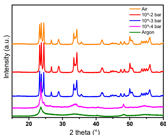
Figure 11. XRD patterns of WO_3 powders synthesized by polyol process and annealed at 600 °C under different oxygen partial pressures: a) under air, b) p(O_2) = 10^{-2} bar, c) p(O_2) = 10^{-3} bar, d) p(O_2) = 10^{-4} bar, e) under argon.
