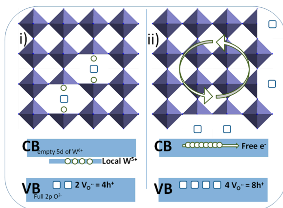
Figure 7. Schematic representation of the blue and the black samples, with simplified crystallographic representation and associated energy band diagrams.
