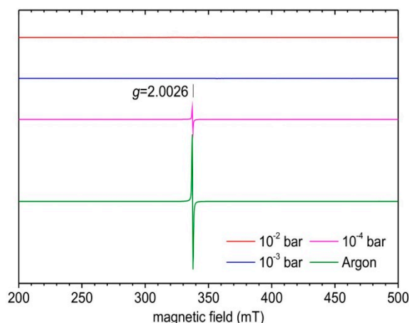
Figure 12. Low-temperature X-band EPR spectra of the samples obtained after different post-annealing treatment at 600 °C.
