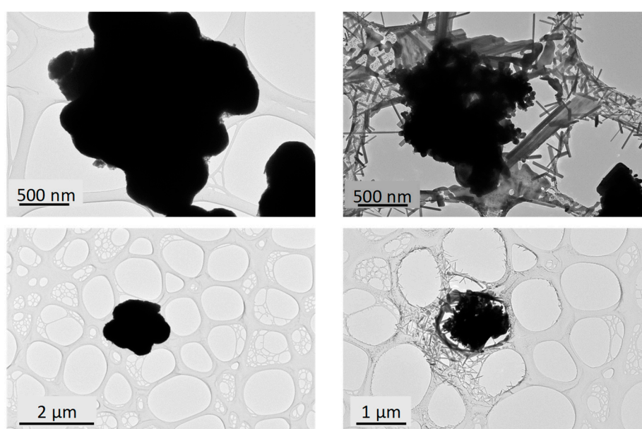
Figure 4. TEM images of \text{WO}_3 black sample just at the beginning of the observation (left panel) and after a few minutes of electron irradiation (right panel).
