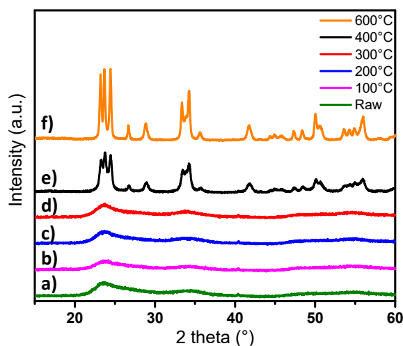
Figure 9. XRD patterns of \text{WO}_3 synthesized by polyol process annealed under air at different temperatures: a) raw blue sample, b) 100, c) 200, d) 300, e) 400 and f) 600 °C.
