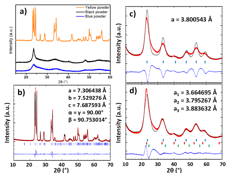
Figure 2. a) X-ray patterns of the blue, black and yellow samples; b) pattern matching refinement for the yellow sample considering a monoclinic phase; c) pattern matching refinement for the blue sample with one cubic unit-cell; d) pattern matching refinement for the blue sample with three superimposed cubic unit-cells.
