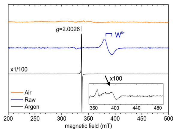
Figure 6. Low temperature (5 K) X-band EPR spectra of raw and annealed (under air or argon) \text{WO}_3 powders.
