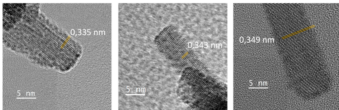
Figure 5. HR-TEM images of some created rod-like crystallite of the \text{WO}_3 black sample after few minutes of electron irradiation.
