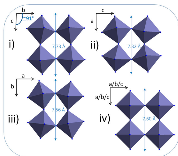
Figure 1. Representation of the octahedral site framework along a , b and c axis projection in the tungsten trioxide ( WO_3 ) monoclinic cell (i–iii), and average pseudo-cubic cell equivalent representation (iv).
