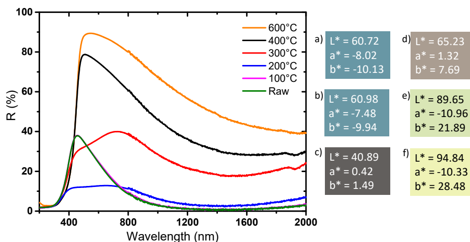
Figure 10. Diffuse reflectance and L^*a^*b^* coloration parameters of the powders annealed under air at different temperatures: a) raw, b) 100, c) 200, d) 300, e) 400 and f) 600 °C.
