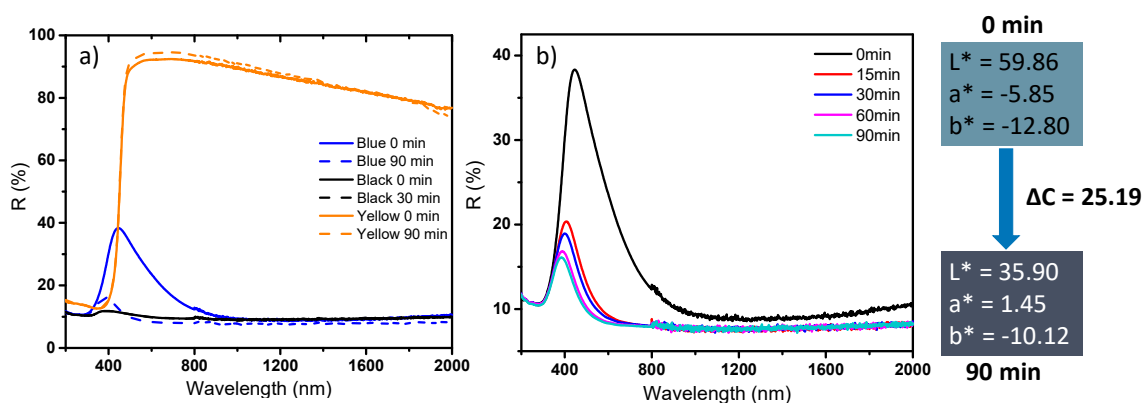
Figure 14. Photochromic behavior of the black, the blue and the yellow sample after different UV (254 nm) irradiation times. a) Comparison of the three samples before irradiation and after 90 min irradiation. b) Kinetic study of the photochromic behavior of the blue sample.
