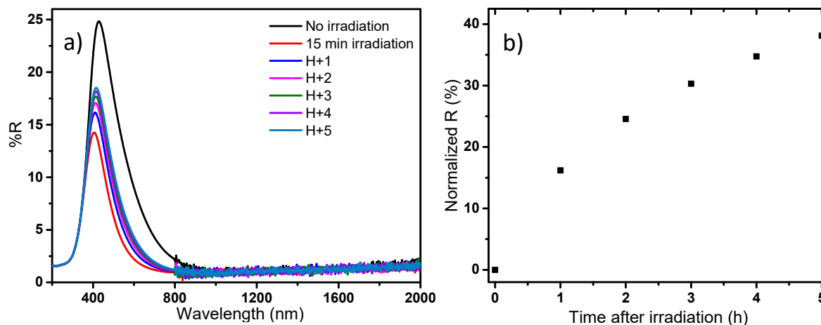
Figure 16. Reversibility of the photochromic behavior of the blue sample after 15 min (254 nm) irradiation time: a) reflectance spectra for different times after irradiation; b) evolution of the normalized reflectance at 500 nm versus time after irradiation.
