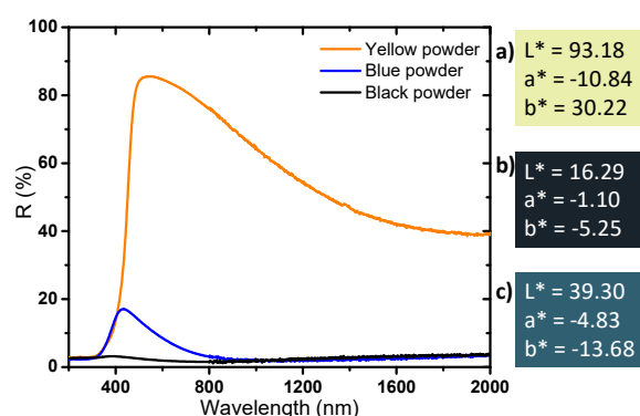
Figure 8. Diffuse reflectance of the powders and L^*a^*b^* parameters coloration of the different WO_3 compounds. a) Yellow, b) black, c) blue powder.
