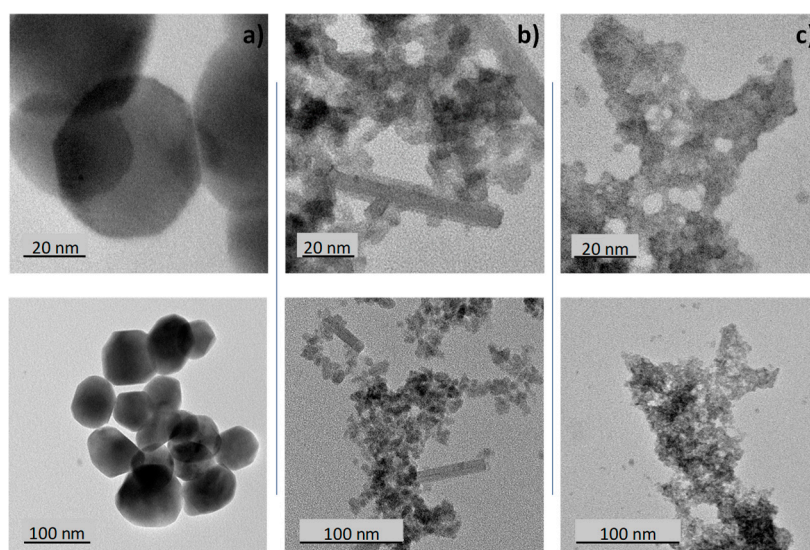
Figure 3. Transmission Electronic Microscopy (TEM) micrographs of \text{WO}_3 powders: a) yellow sample, b) black sample, c) blue sample.
