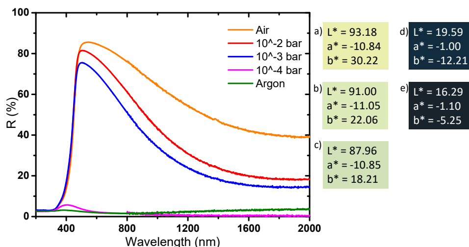
Figure 13. Diffuse reflectance and L^*a^*b^* coloration parameters of the powders annealed at 600 °C under different oxygen partial pressures: a) air, b) 10^{-2} bar c) 10^{-3} bar d) 10^{-4} bar and e) argon.
