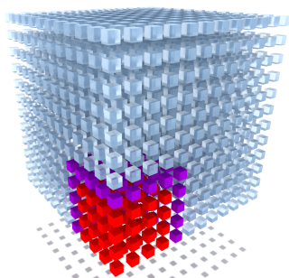
Figure 2: Compute a 4^3 subset (red) of the 12^3 grid. The subset of the grid needs to access a larger part in the distance refinement step (represented here in purple) that has to be computed in the probe intersection step.
