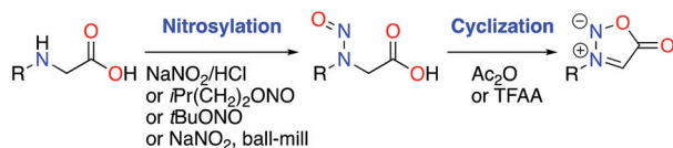
Scheme 1 Different existing synthetic methods for the preparation of sydrones.
