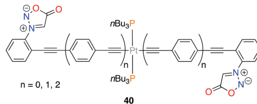
Fig. 2 Formation of syndnone-containing platinum acetylide oligomers.
