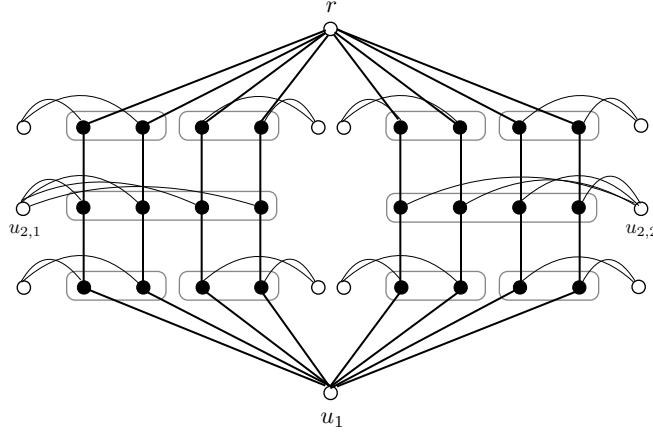
Figure 2: A different construction of the adversarial graph G_2 of Figure 1. Here, only non-solid vertices can be requested as terminals. Solid edges have weight 1/4 , all other edges have 0 weight. Rectangles depict the s -sets to which potentially requested terminals connect. Note that there are 8 columns in total.
