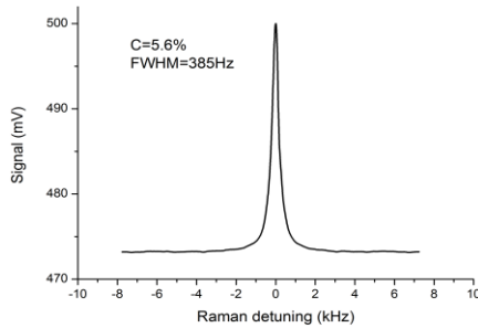
Fig. 6. Typical CPT clock signal.
