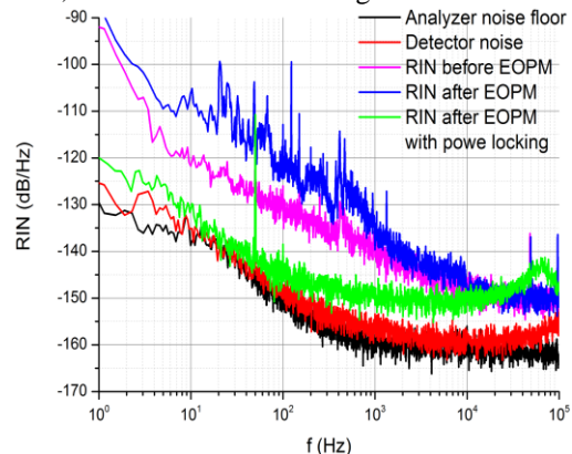
Fig. 2. The laser RIN before and after pass through the EOPM, in the latter case, the RIN with and w/o laser power locking are recorded, the detector noise and analyzer noise floor are also presented.
