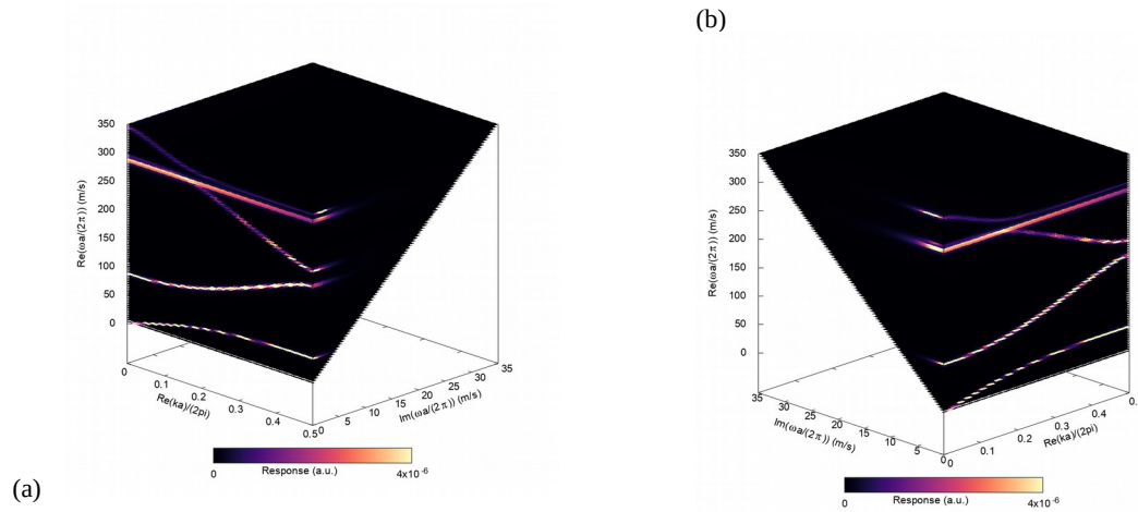
Figure 2: (a-b) Complex resolvent band structure shown for real wavenumber and complex frequency in the case of a lossy sonic crystal of rectangular resonators grafted along an air tube.
