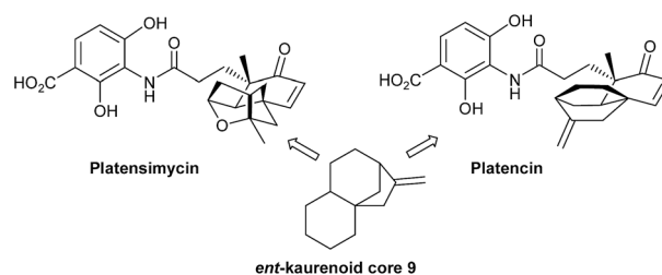
Scheme 4 Ent -kaurenoid biosynthetic precursor of platensimycin and platencin.
