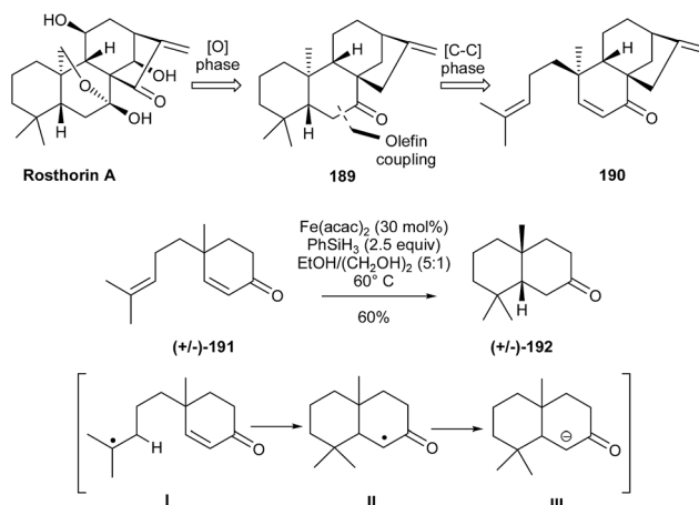
Scheme 46 Baran's general two-phase strategy for elaboration of rosthorin.
