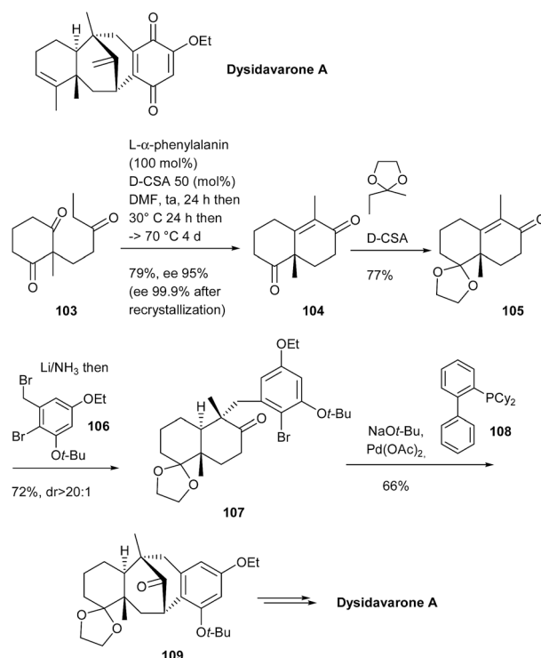
Scheme 27 Menche's total synthesis of dysidavarone A.
