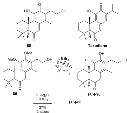
Scheme 23 Yang's total synthesis of an o -hydroxy- p -quinone methide diterpenoid structurally related to taxodione.
