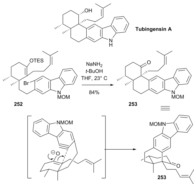
Scheme 58 Garg's total synthesis of (+)-tubingensin A.
