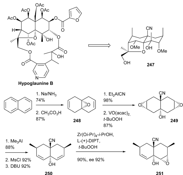
Scheme 57 Spivey's approach towards hypoglaunine B.
