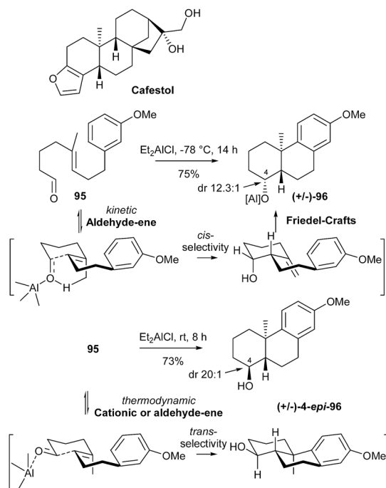
Scheme 25 Hong's total synthesis of ( \pm )-cafestol.
