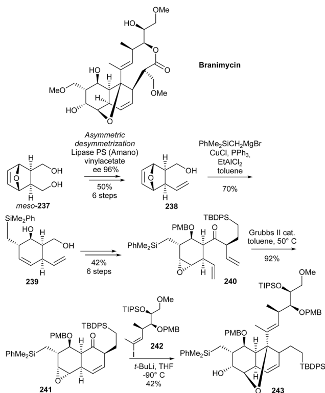
Scheme 55 Mulzer's synthesis of the cis -decalin core of branimycin.
