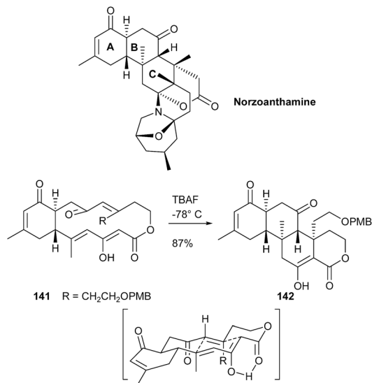
Scheme 35 Yang's synthesis of the ABC carbocyclic core of norzoanthamine by transannular Michael reaction cascade.
