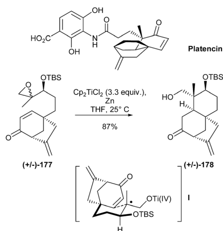
Scheme 43 Yoshimitsu's synthesis of ( \pm )-platencin.
