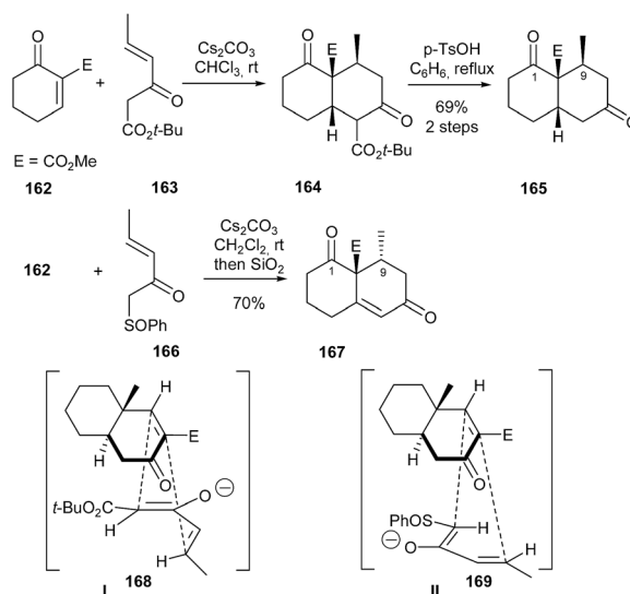
Scheme 40 Deslongchamps' “anionic Diels–Alder reaction”.
