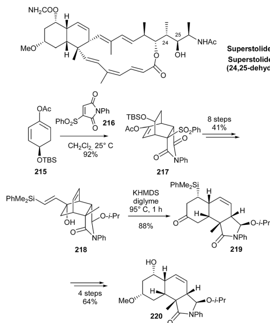
Scheme 51 Jin's synthesis of the cis -decalin core superstolides A and B.
