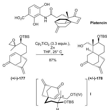
Scheme 43 Yoshimitsu's synthesis of (±)-platencin.
