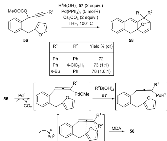
Scheme 12 Intramolecular Diels–Alder reaction of furans.
