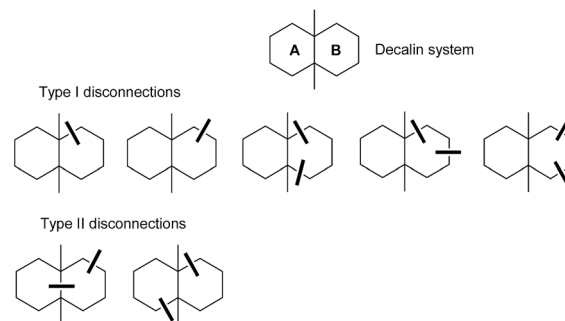
Scheme 1 Decalin synthesis according to type I and II disconnections of the review.
