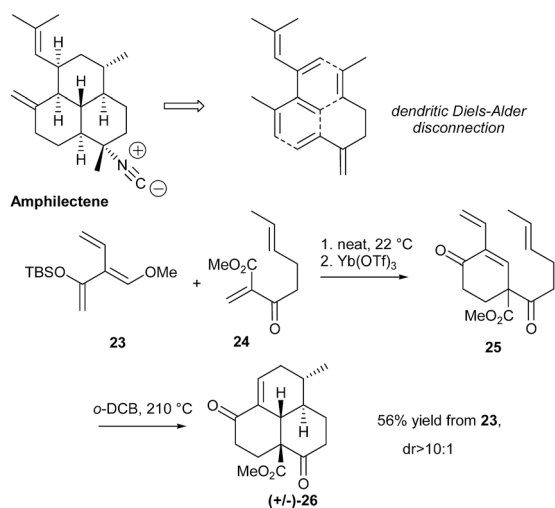
Scheme 7 Shenvi's total synthesis of amphilectene.
