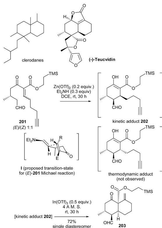
Scheme 48 Lee's total synthesis of (–)-teuvidin.
