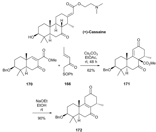
Scheme 41 Deslongchamps' synthesis of (+)-cassaine.
