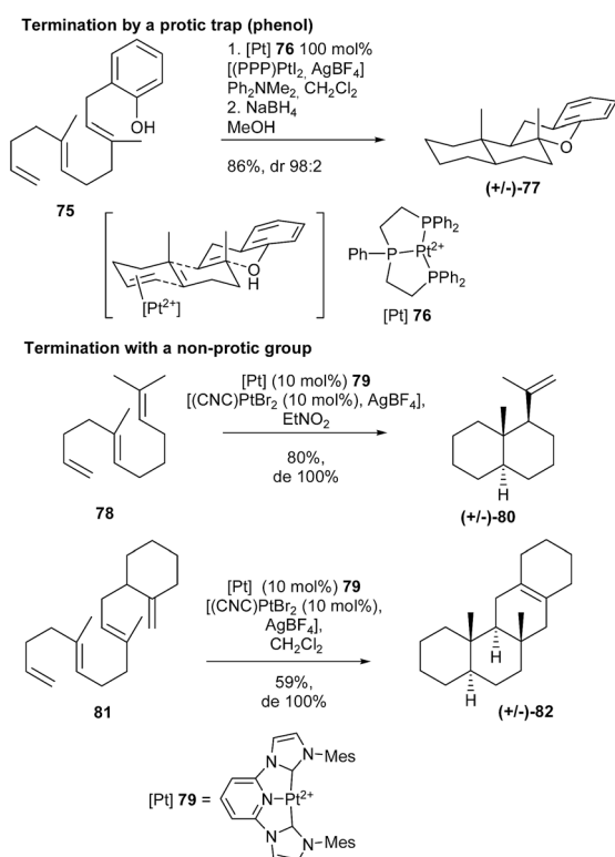
Scheme 20 Gagné's platinum catalyzed cascade cyclization of polyenic systems.
