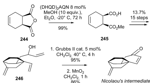
Scheme 56 Lee's synthesis of the Nicolaou's intermediate of platencin.
