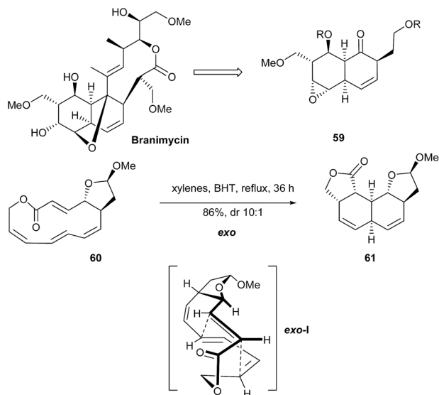
Scheme 14 Mulzer's synthetic approach to branimycin.
