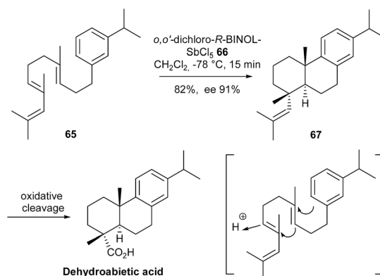
Scheme 16 Corey's total synthesis of dehydroabietic acid.
