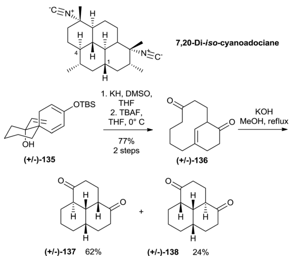
Scheme 33 Vanderwal's approach to 7,20-di-iso-cyanoadociane.
