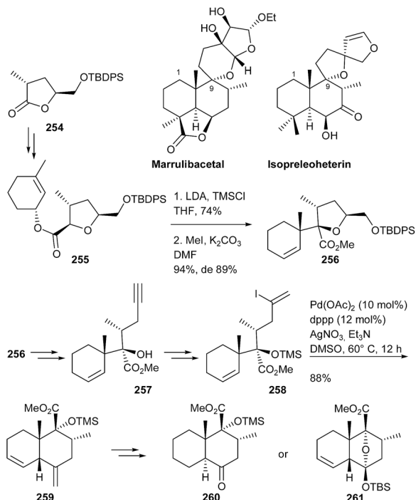
Scheme 59 Nakamura's approach towards C9-oxygenated labdane diterpenoids.
