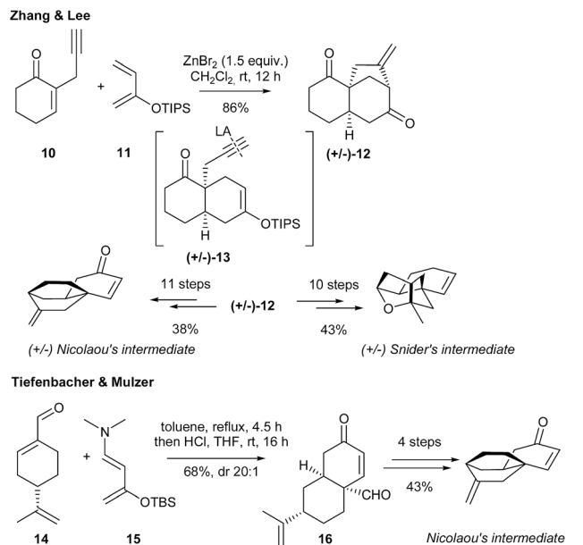
Scheme 5 Zhang, Lee, Tiefenbacher and Mulzer syntheses of Nicolaou and Snider intermediates of platencin and platensimycin.
