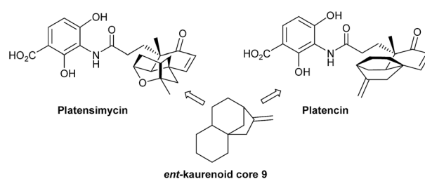
Scheme 4 Ent -kaurenoid biosynthetic precursor of platensimycin and platencin.
