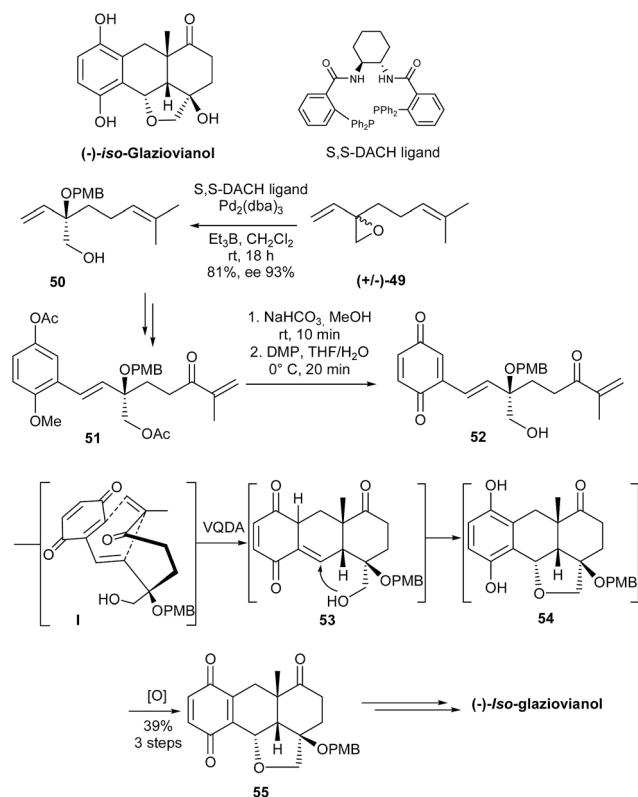
Scheme 11 Trauner's total synthesis of iso-glaziovianol.
