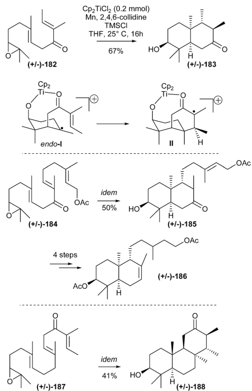
Scheme 45 Cuerva's Ti(III)-catalyzed radical cyclization of epoxy polyenes with keto units.
