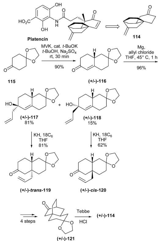
Scheme 29 Yadav's total synthesis of the bridged tricyclic core of racemic platencin.
