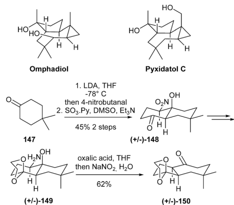
Scheme 37 Liang's total synthesis of racemic omphadiol and pyxidatol C.
