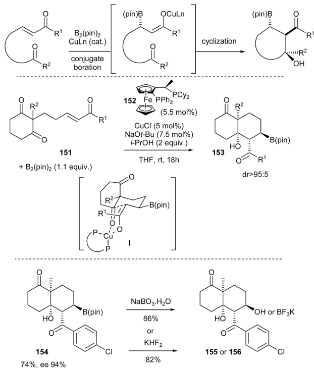
Scheme 38 Lam's borylative aldol cyclization of enones.
