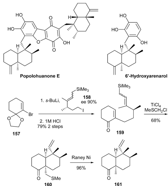
Scheme 39 Anderson's synthesis of 6'-hydroxyarenarol, precursor of popolohuanone E.
