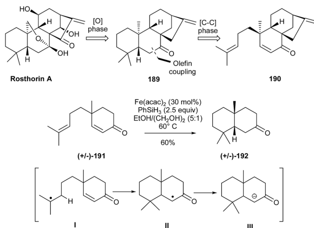
Scheme 46 Baran's general two-phase strategy for elaboration of rosthoin.
