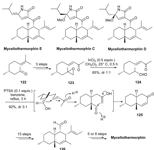
Scheme 30 Nicolaou's total synthesis of myceliothermorphins.
