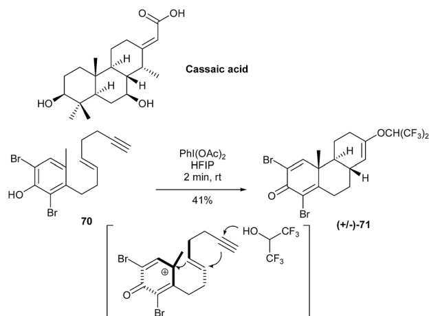
Scheme 18 Canesi's oxidative cationic polycyclization process.
