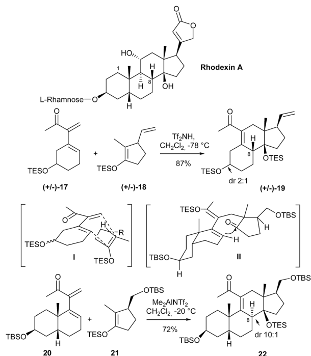
Scheme 6 Hindered inverse-electron-demand DA reaction towards rhodexin synthesis.
