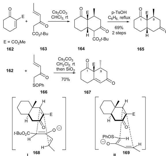
Scheme 40 Deslongchamps' “anionic Diels–Alder reaction”.
