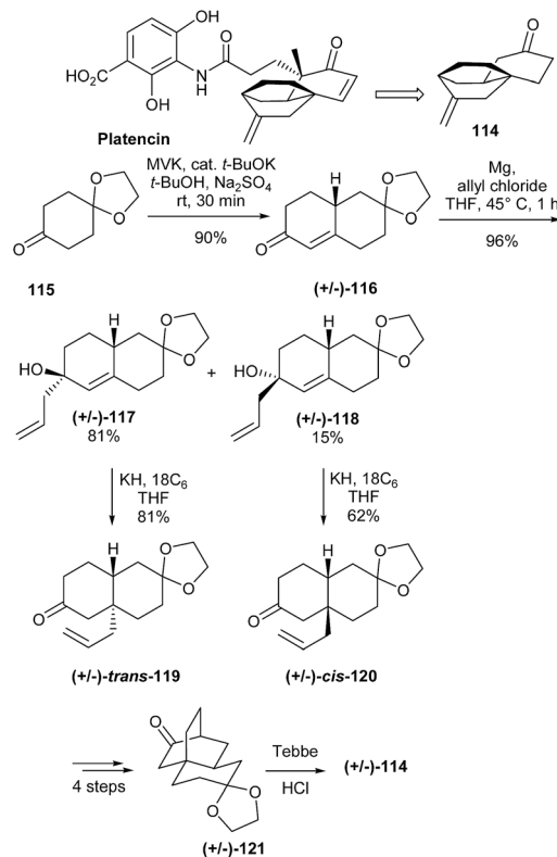
Scheme 29 Yadav's total synthesis of the bridged tricyclic core of racemic platencin.
