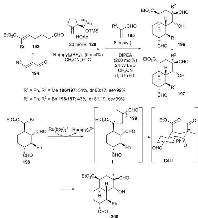
Scheme 47 Hong's strategy for the enantioselective synthesis of highly functionalized decalins.
