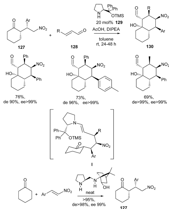
Scheme 31 Chen's organocatalytic reaction of \gamma -nitroketones with \alpha,\beta -unsaturated aldehydes.
