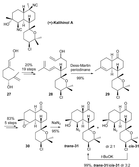
Scheme 8 Miyaoka's total synthesis of kalihinol.
