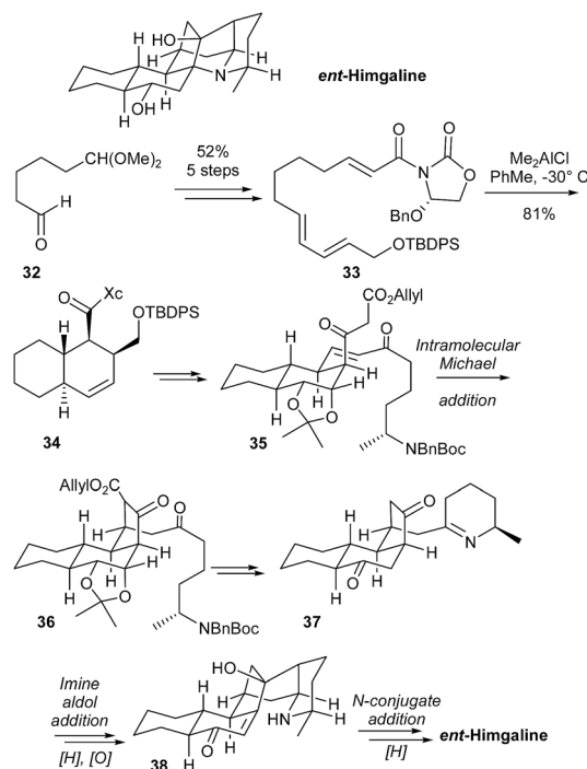
Scheme 9 Evans' total synthesis of ent -himgaline.
