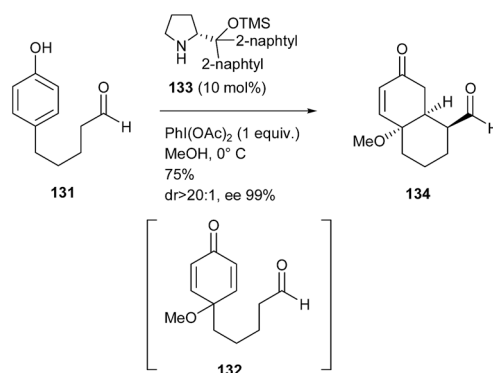
Scheme 32 Gaunt's one-pot oxidative dearomatization of phenols and asymmetric intramolecular Michael addition.
