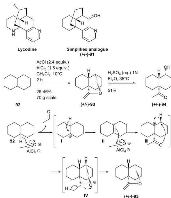
Scheme 24 Lewis' “aliphatic Friedel–Crafts” approach.
