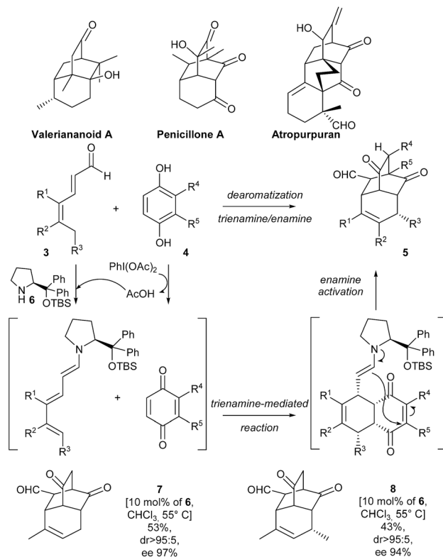
Scheme 3 Greck's method for formation of tricyclic ring systems.
