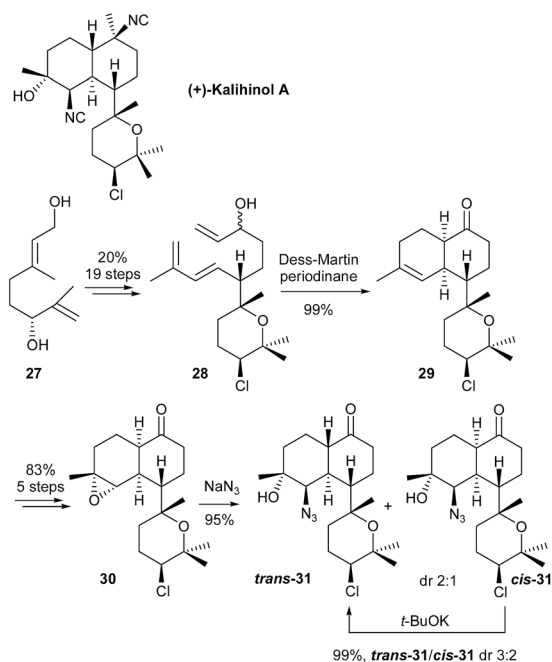
Scheme 8 Miyaoka's total synthesis of kalihinol.
