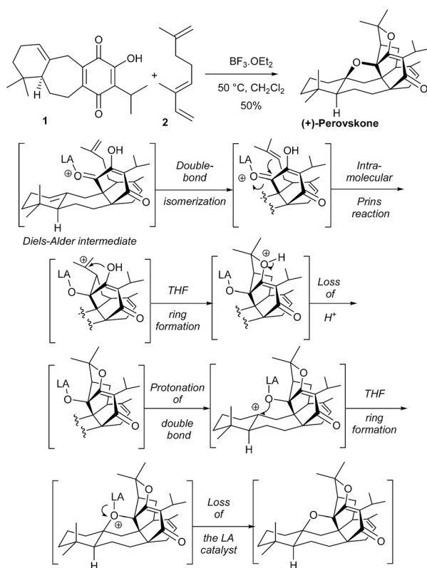
Scheme 2 Majetich's total synthesis of perovskone.
