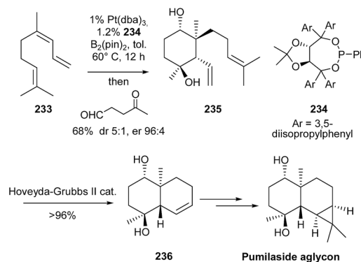
Scheme 54 Morken's synthesis of the aglycon of pumilaside.
