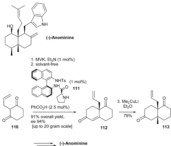
Scheme 28 Bradshaw and Bonjoch total synthesis of (-)-anominine.
