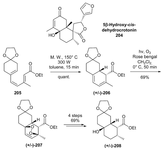
Scheme 49 Williams' synthesis of the cis -hydroxydecalin system of crotonin.
