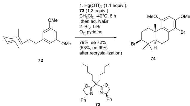
Scheme 19 Snyder's asymmetric halonium-induced cation- \pi cyclization.
