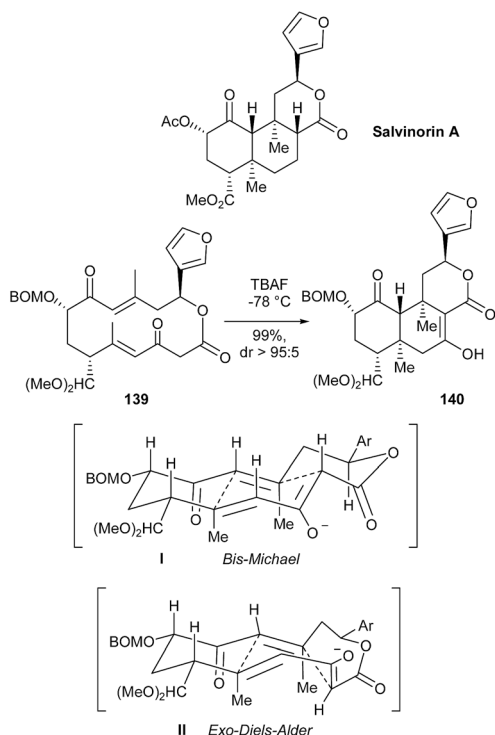
Scheme 34 Evans's synthesis of salvinorin A by transannular Michael reaction cascade.
