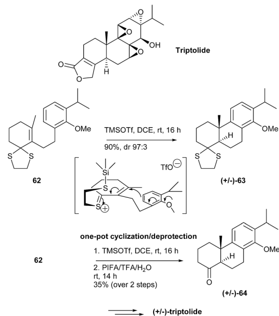
Scheme 15 Baati's total synthesis of racemic triptolide.
