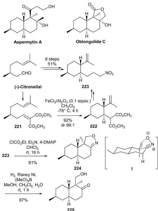
Scheme 52 Yoshida and Shishido synthesis of aspermytin A and oblongolide C.
