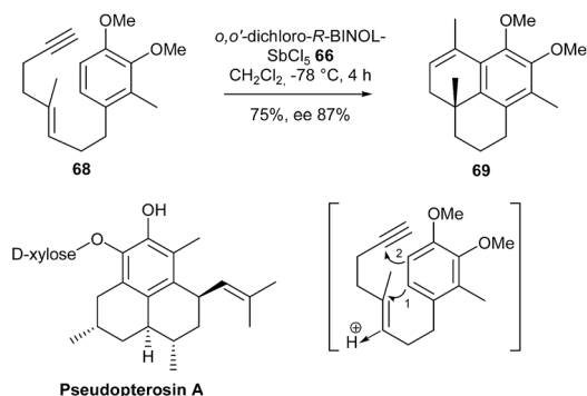
Scheme 17 Corey's synthesis of analogue of pseudopterosin.
