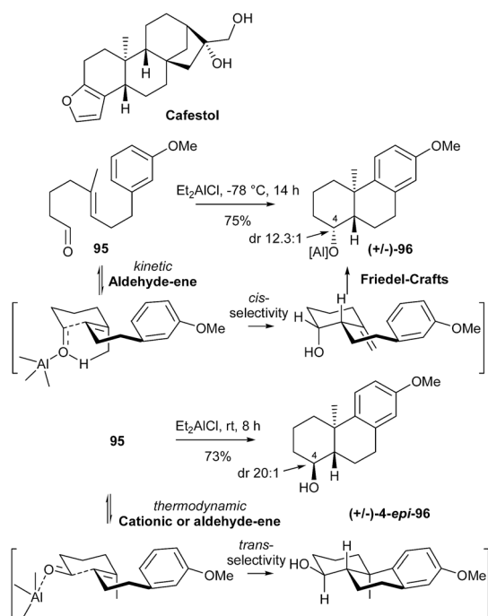
Scheme 25 Hong's total synthesis of (±)-cafestol.
