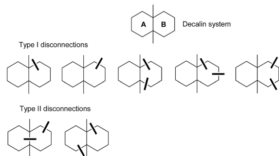
Scheme 1 Decalin synthesis according to type I and II disconnections of the review.
