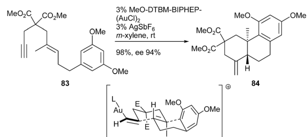
Scheme 21 Toste's polycyclization reactions.
