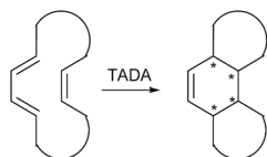
Scheme 13 General scheme for TADA reactions.
