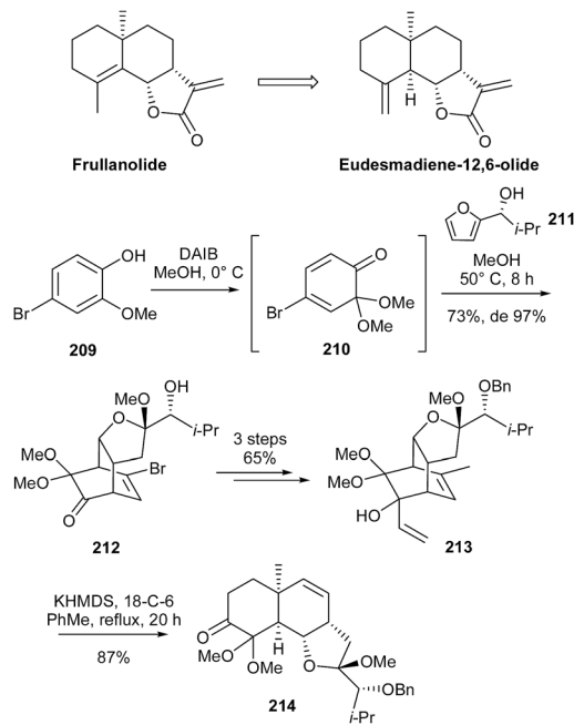
Scheme 50 Liao's total synthesis of eudesmadiene-12,6-olide and frullanolide.
