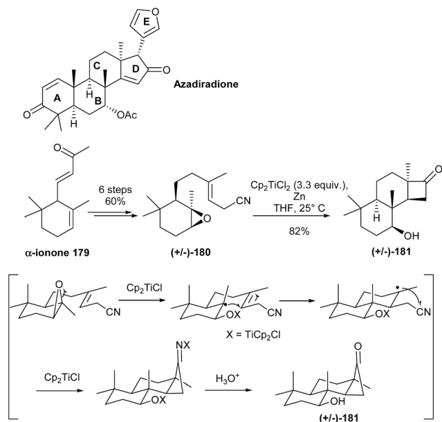
Scheme 44 Fernández-Mateos' synthesis of the BCDE core of azadiradione.
