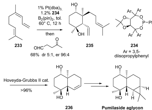
Scheme 54 Morcken's synthesis of the aglycon of pumilaside.
