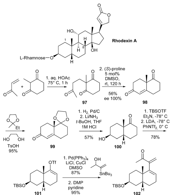
Scheme 26 Jung's Wieland–Miescher ketone strategy towards rhodexin.
