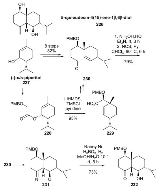
Scheme 53 Kündig's synthesis of eudesmane.
