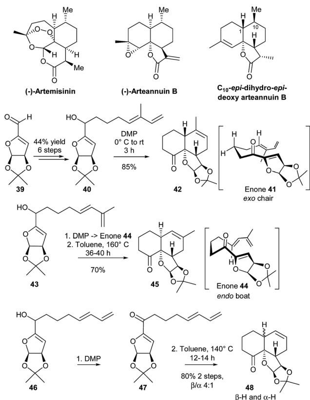
Scheme 10 Gosh's total synthesis of C 10 -epi-dihydro-epi-deoxy arteannuin B.
