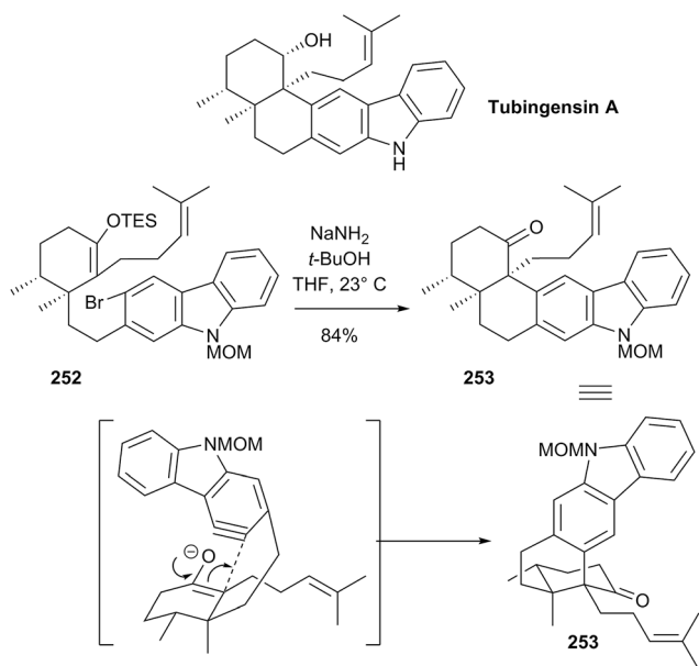
Scheme 58 Garg's total synthesis of (+)-tubingsensin A.
