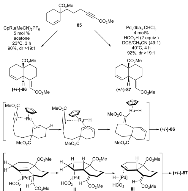
Scheme 22 Trost's cycloisomerization of enynes containing cyclic olefins.
