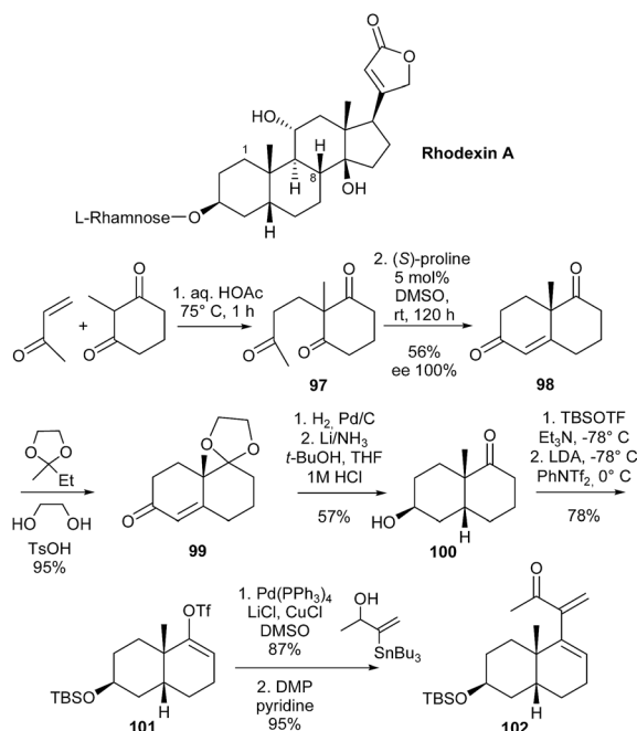
Scheme 26 Jung's Wieland–Miescher ketone strategy towards rhodexin.
