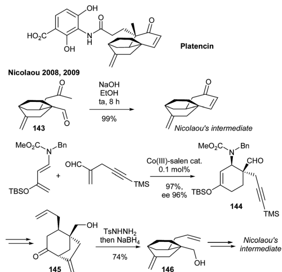
Scheme 36 Nicolaou's synthesis of platencin by intramolecular aldol reaction.
