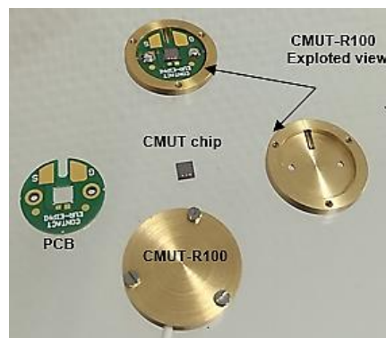
Figure 2: Prototype CMUT-R100
