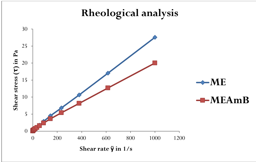
Figure 3: Rheological behavior of ME and ME containing AmB.
