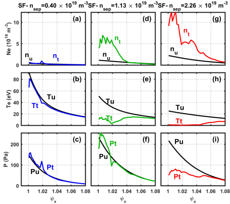
Figure 7. Comparison of density, temperature, and pressure profiles at the upstream (midplane) and the outer target versus increasing densities for SF-configuration. The left column corresponds to the lowest separatrix density, as well as the blue shaded region in figure 6. The middle and right column correspond to intermediate and highest densities, also to the same color shaded region in figure 6.
