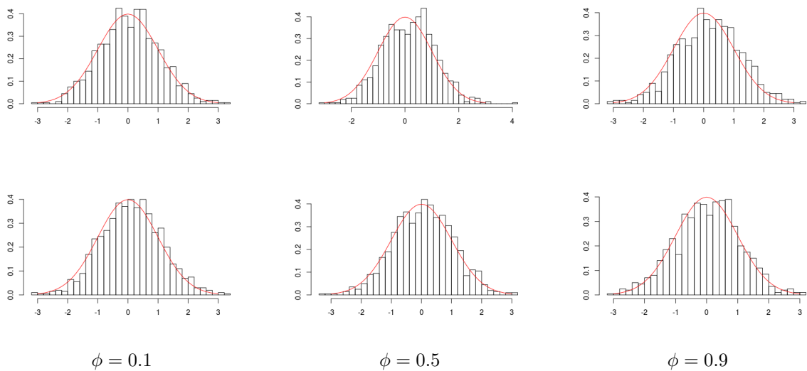
FIGURE 22. Histograms for c = 5 , d = -5 , n = 1000 . First row: (\widehat{c}_n^{(1)} - c) . Second row: (\widehat{d}_n^{(1)} - d) .
