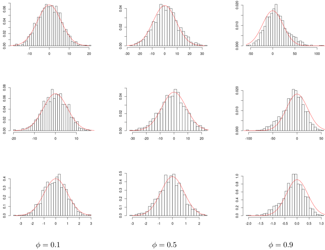
FIGURE 21. Histograms for a = 5 , b = -5 . First row: (\widehat{m}_n^{(1)} - m) . Second row: (\widehat{b}_n^{(1)} - b) . Third row: (\widehat{\phi}_n^{(1)} - \phi) .
